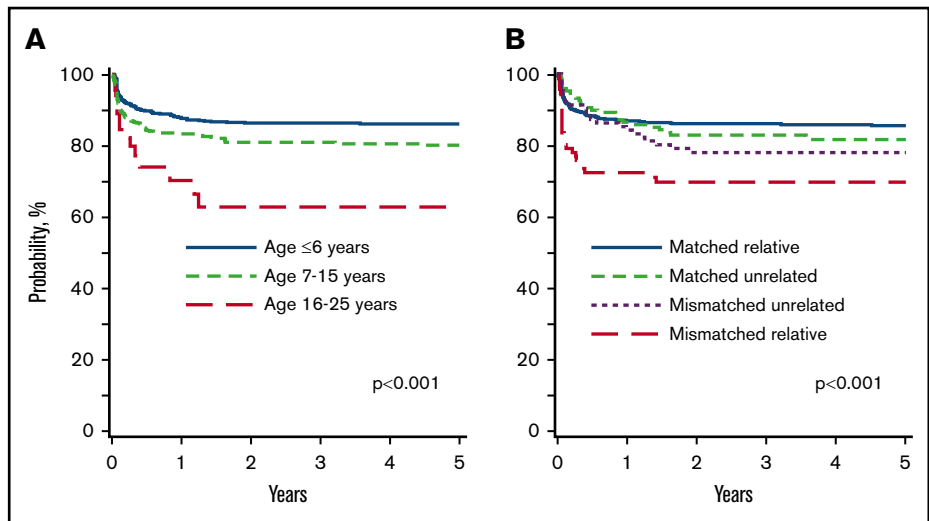
Figure 1. Event-free survival. (A) Event-free survival by age at transplantation. The 5-year probabilities of event-free survival for patients aged \leq 6 years, 7 to 15 years, and 16 to 25 years were 86% (83% to 89%), 80% (76% to 84%), and 63% (48% to 78%), respectively. (B) Event-free survival by donor type. The 5-year probabilities of event-free survival after HLA-matched relative, HLA-mismatched relative, HLA-matched unrelated, and HLA-mismatched unrelated donor transplants were 86% (83% to 88%), 70% (61% to 79%), 82% (75% to 89%), and 78% (70% to 86%), respectively.
