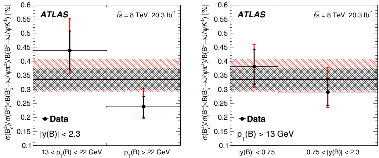
FIG. 7. Summary of the cross-section measurement presented in this article. The left figure shows the production cross section for the B_c^\pm relative to the B^\pm (times the corresponding branching fractions) for two bins in p_T (black data points) and for the inclusive bin (horizontal band). The right figure shows the measurement binned in rapidity (black data points). On each point the horizontal bar indicates the bin width. The vertical inner error bars on the data points indicate the statistical uncertainty. The outer error bars indicate the size of the quadrature sum of uncertainties from all sources: statistical, systematic, and lifetime. The double hatched error band indicates statistical uncertainty, while the single hatched bands indicate the quadrature sum of uncertainties from all sources.
