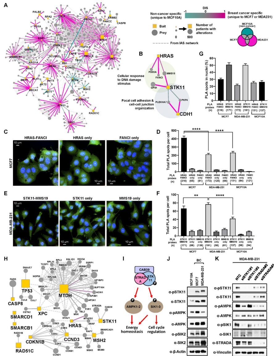
Figure 2. Differential interaction analysis of the BC-enriched interactome.
