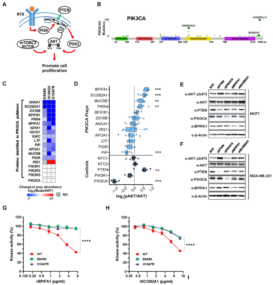
Figure 3. Comparative interactome analysis of WT and mutant PIK3CA proteins.
