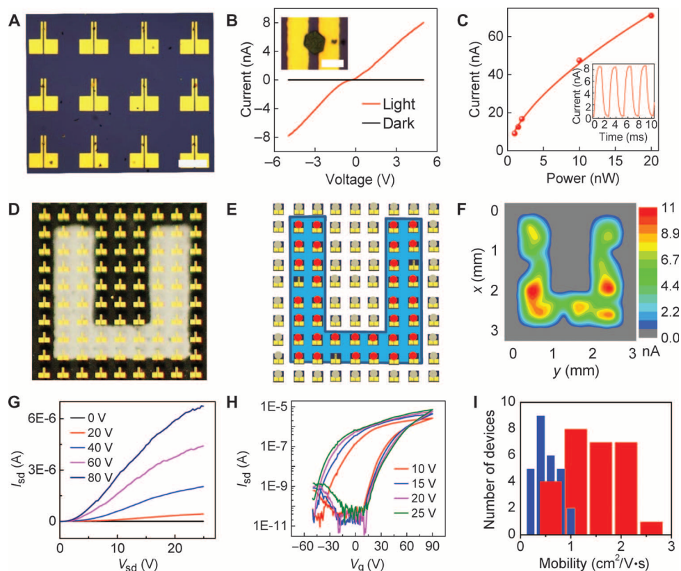
Fig. 4. Selective growth of perovskite crystals on prepatterned electrodes for photodetector arrays and FETs. (A) Optical microscopy image of perovskite microplate crystals bridging prepatterned arrays of electrode pairs. Scale bar, 200 \mu\text{m} . (B) Typical I - V curve of a perovskite crystal under dark and light illumination. (Inset) Optical microscopy image of a perovskite crystal bridging two gold electrodes. The distance between the electrode pair is 8 \mu\text{m} . Scale bar, 20 \mu\text{m} . (C) Photocurrent versus incident light power of a typical device (source-drain voltage, 5 V). (Inset) Response speed of a typical two-probe device (laser illumination, 488 nm; power, 1.2 nW; source-drain voltage, 5 V). (D) Optical image of photodetector arrays with a U-shaped mask (U-shaped transparent area). (E) Schematic illustration of the device arrangement of photodetector arrays with a U-shaped mask under blue LED illumination (wavelength, 463 nm; power density, 600 \mu\text{W}/\text{cm}^2 ). Red dots, devices with photocurrent; gray dots, devices without photocurrent. (F) Photocurrent mapping of photodetector arrays with a U-shaped mask under blue LED illumination. (G and H) Output ( V_g = 0, 20, 40, 60, and 80 V) (G) and transfer ( V_{sd} = 10, 15, 20, and 25 V) (H) characteristics of FET based on a perovskite microplate crystal at 77 K. (I) Distribution of the field effect electron mobility of 27 perovskite microplate transistors measured at 77 K. Red, mobility derived from backward sweep; blue, mobility derived from forward sweep.
