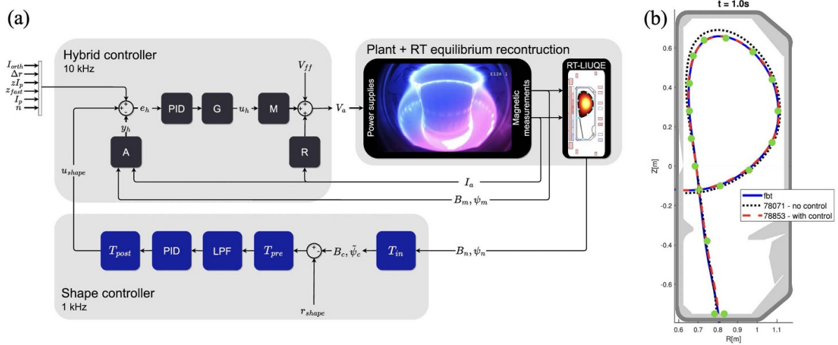
Figure 12. (a): Block diagram of the TCV magnetic control architecture. (b): Comparison of the programmed plasma boundary (solid blue) with discharge 78 071 without shape control (black dotted) and discharge 78 853 with shape control (red dashed) at t = 1.0 s. Reproduced from [101]. © The Author(s). Published by IOP Publishing Ltd. CC BY 4.0.
