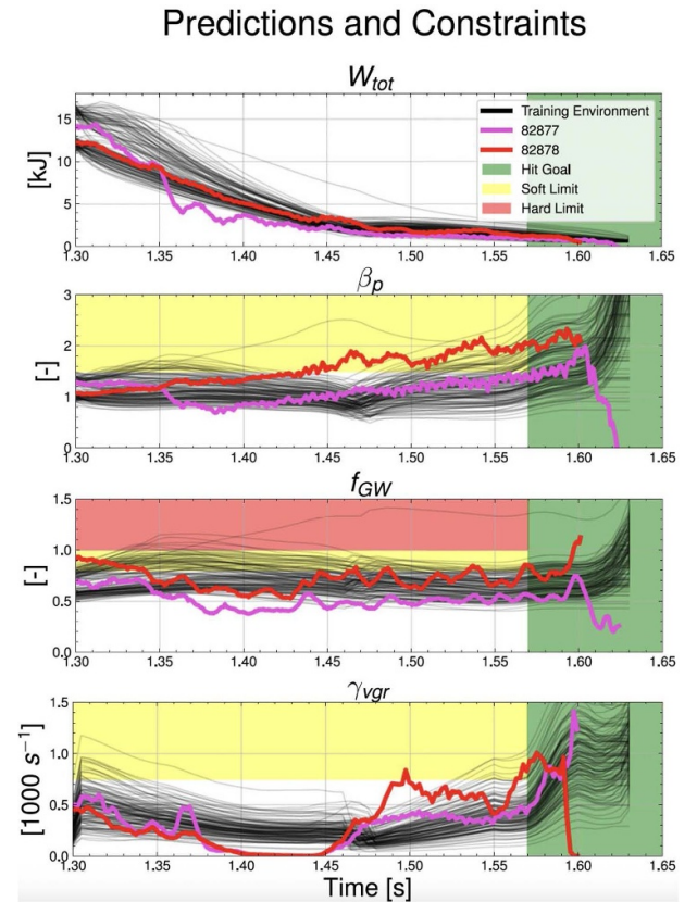
Figure 13. Predictions and experimental results of rampdown trajectories based on Scientific Machine Learning, for a high-performance discharge with plasma current extrapolation, demonstrating successful plasma termination. Shown are the experimental time traces of stored energy, plasma beta, Greenwald fraction, and vertical growth rate, together with the a priori predictions (black curves). Reproduced from [124]. CC BY 4.0.
