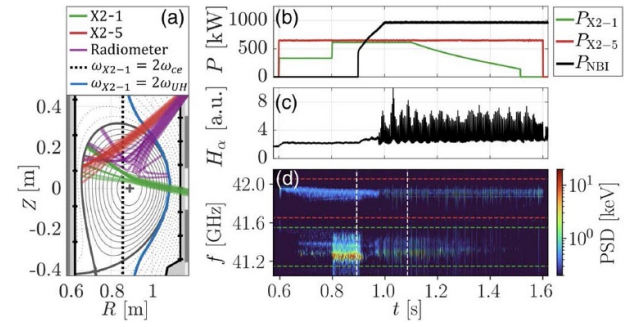
Figure 7. (a) Poloidal cross section of a TCV discharge with resonances, gyrotron ray trajectories, and line of sight of the radiometer overlaid. (b) and (c) Time traces of the injected power and H_\alpha signal, with the latter highlighting the transition to H-mode following NBI injection. (d) Frequency spectrum of the radiometer, showing a clear signal at half frequency of both the X2-1 gyrotron (41.35 GHz, indicated by the green band) and the X2-5 gyrotron (41.90 GHz, indicated by the red band) as a result of a Two-Plasmon Decay Instability (TPDI), with different characteristics in the L-mode and H-mode phases of the shot. Reprinted figure with permission from [64], Copyright (2024) by the American Physical Society.
