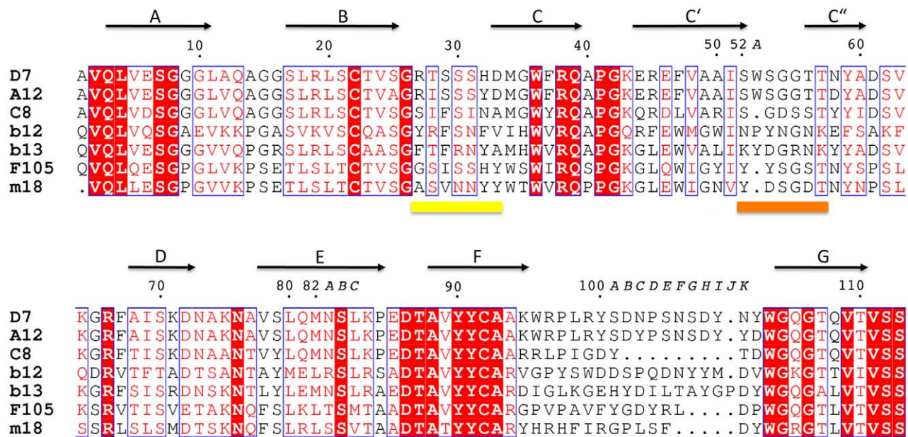
Figure 2. Structure based sequence alignment of D7 with V HH A12 and C8 as well as with the V H domains from the neutralizing antibodies b12, b13, F105 and m18. The residue numbering is according to Chothia [38] and the CDRs are indicated by coloured bars.
