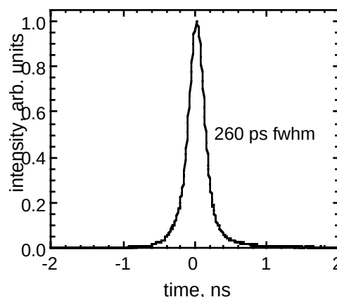
Fig. 4. Timing resolution spectrum measured for a LaBr 3 :Ce (5% Ce 3+ ) crystal in coincidence with a BaF 2 crystal.
