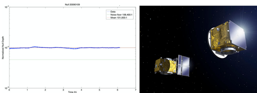
Fig. 9 Left: 6-h measurement of the null-depth achieved at 10\ \mu\text{m} wavelength with the “Adaptive Nuller” at JPL [68]. Right: Artist impression of ESA’s PROBA 3 spacecraft, the first mission to demonstrate autonomous precision formation flying (Image credit: ESA - P. Carril, 2013)
