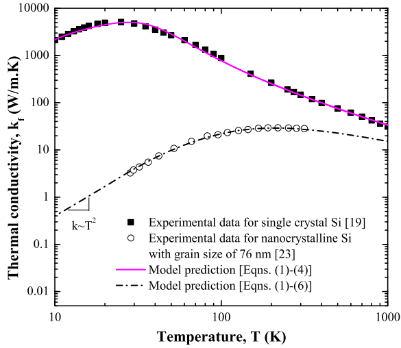
FIGURE 3. Thermal conductivity reported in the literature for high purity single crystal silicon [19] and dense nanocrystalline silicon [23] as a function of temperature. The solid and dashed lines correspond to the model predictions from the kinetic theory model [Equations (1) to (6)] for single crystal and nanocrystalline silicon, respectively.
