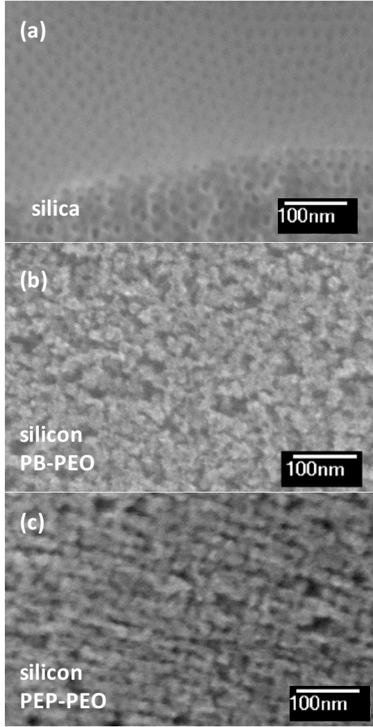
FIGURE 2. Top surface SEM images of (a) a PEP-PEO templated mesoporous silica film, (b) a PB-PEO templated silicon film after magnesium treatment and HCl and HF washes, and (c) a PEP-PEO templated silicon film after magnesium treatment and HCl and HF washes.
