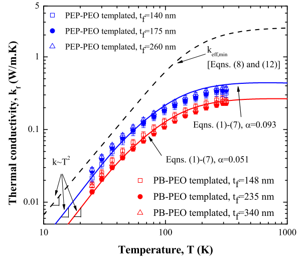
FIGURE 4. Measured thermal conductivity of mesoporous silicon thin films as a function of temperature from 25 to 315 K. The lines correspond to the model predictions from the kinetic theory model [Equations (1) to (7)] and the effective minimum thermal conductivity model [Equations (8) and (12)].
