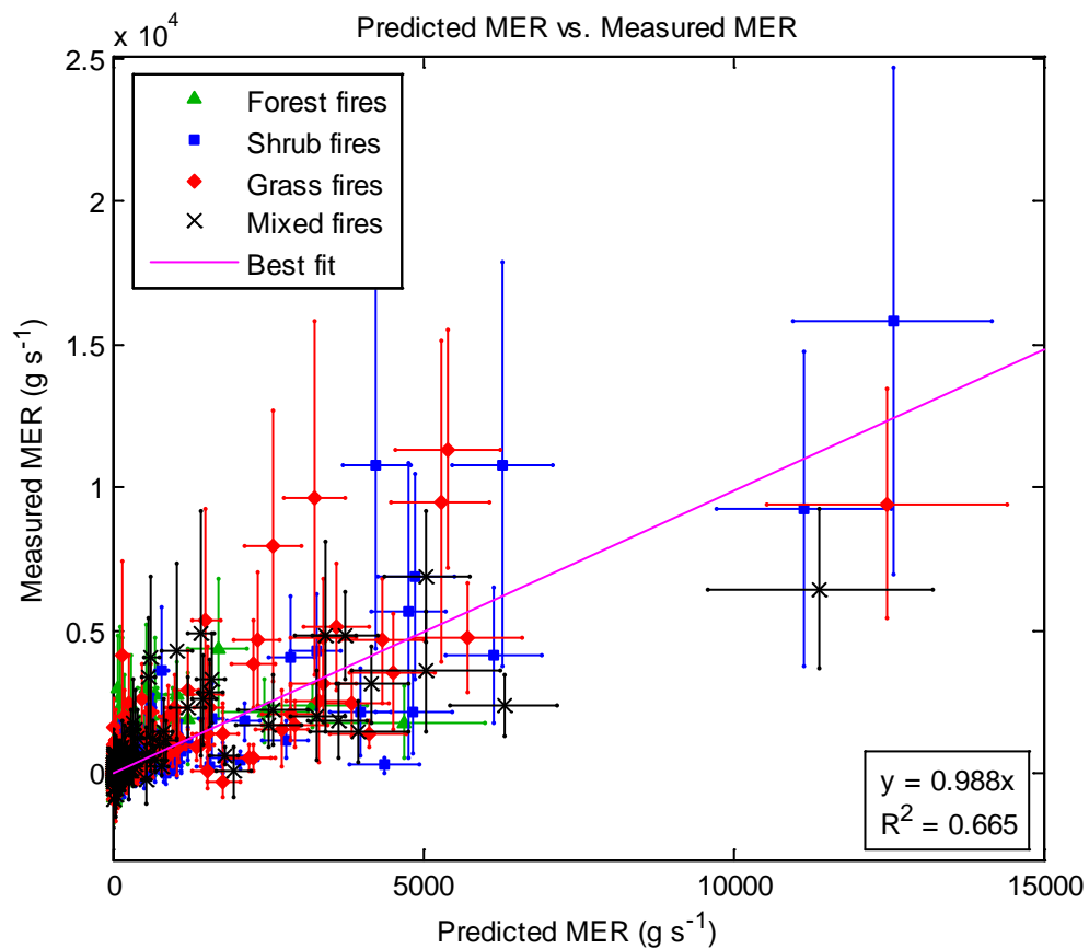
Figure 2.4. Predicted NO 2 mass emission rate (MER), calculated using fire radiative power and the multiple regression coefficients, vs. MER measured in the analysis. Error bars in measured MER are one standard deviation, calculated as reported; error bars in predicted MER are calculated using one standard deviation of each calculated emission coefficient.
