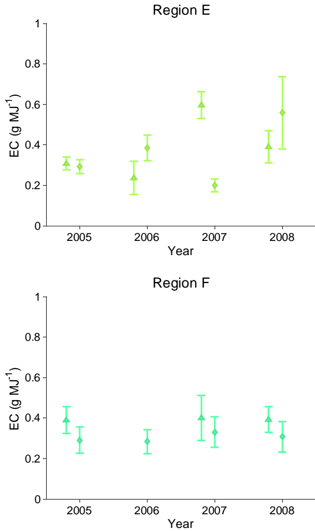
Figure 6.2. ECs calculated by year (2005-2008) and biome for Regions E and F, both mixed tropical-temperate forests. Triangles indicate ECs for tropical forests, while diamonds indicate ECs for temperate forests. In Region E, interannual variability in ECs varies significantly for the two biomes, while in Region F the interannual variability is small and is similar between the two biomes.
