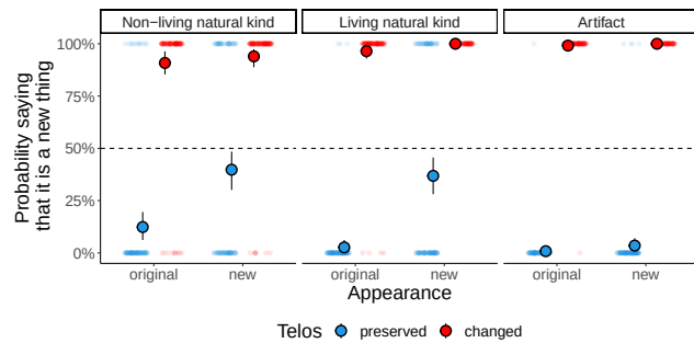
(a) GPT-3 Telos vs. Appearance
