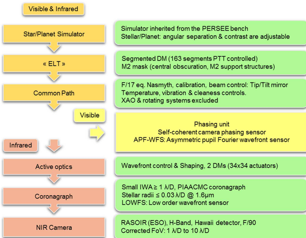
Figure 2. General layout.
