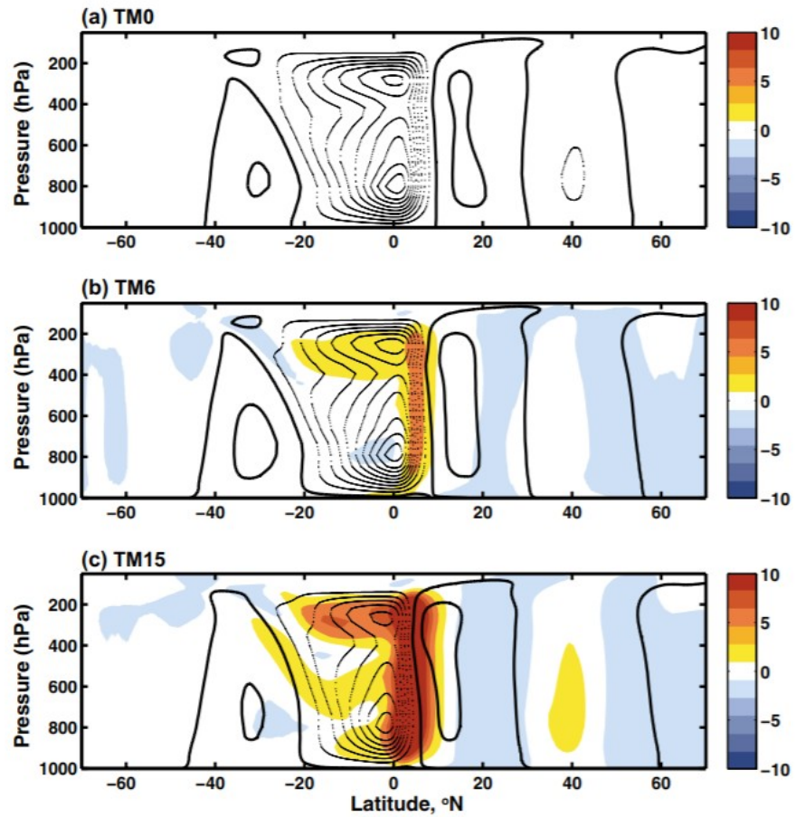
Fig. 3 Zonally-averaged stream function for TM0 (black solid and dashed contours indicating positive and negative values with 5 \times 10^{10} \text{ kg s}^{-1} contour interval) and corresponding anomalies (colors, units of 10^{10} \text{ kg s}^{-1} ) in a TM0, b TM6, and c TM15. The stream function anomalies imply the southward shift of the Hadley circulation and a weakening of the winter Hadley cell in the warmer climates
