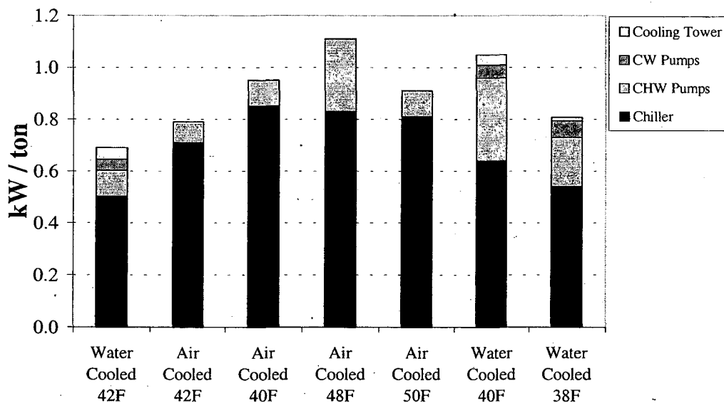
Figure 7. Chilled water system comparison.
