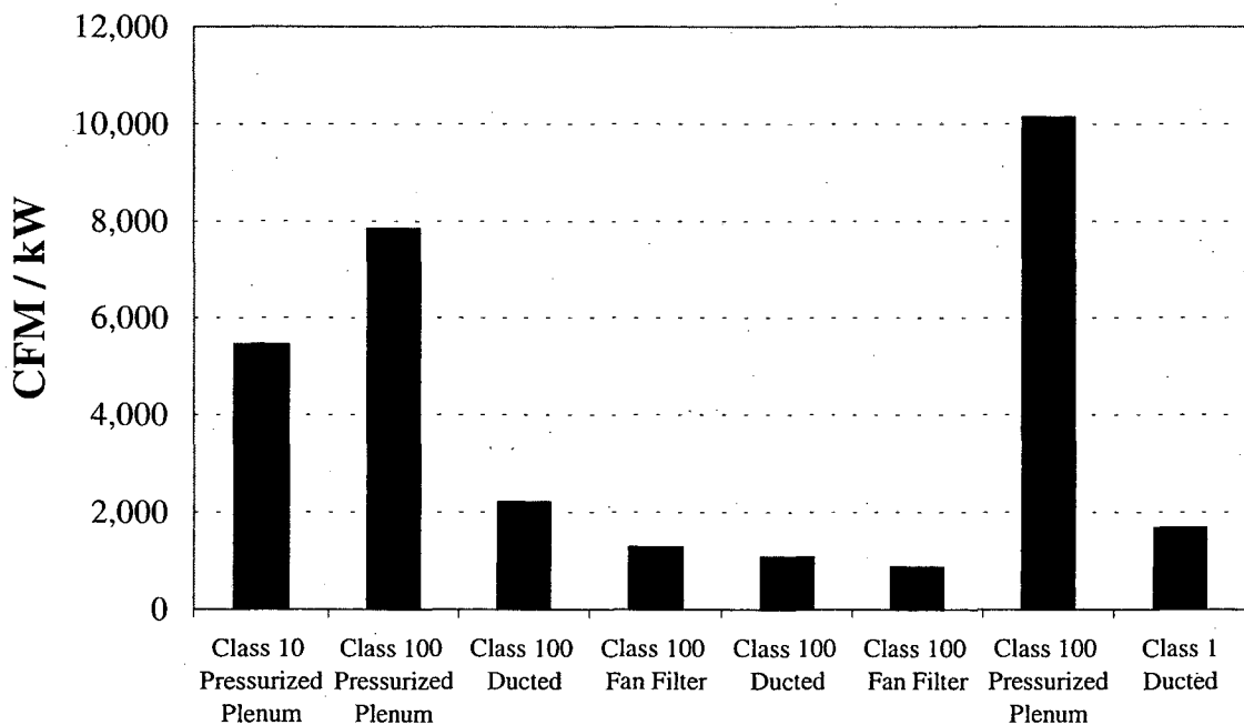
Figure 3. Cleanroom air circulation system efficiency.
