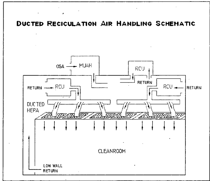
Figure 5. Ducted recirculation system.
