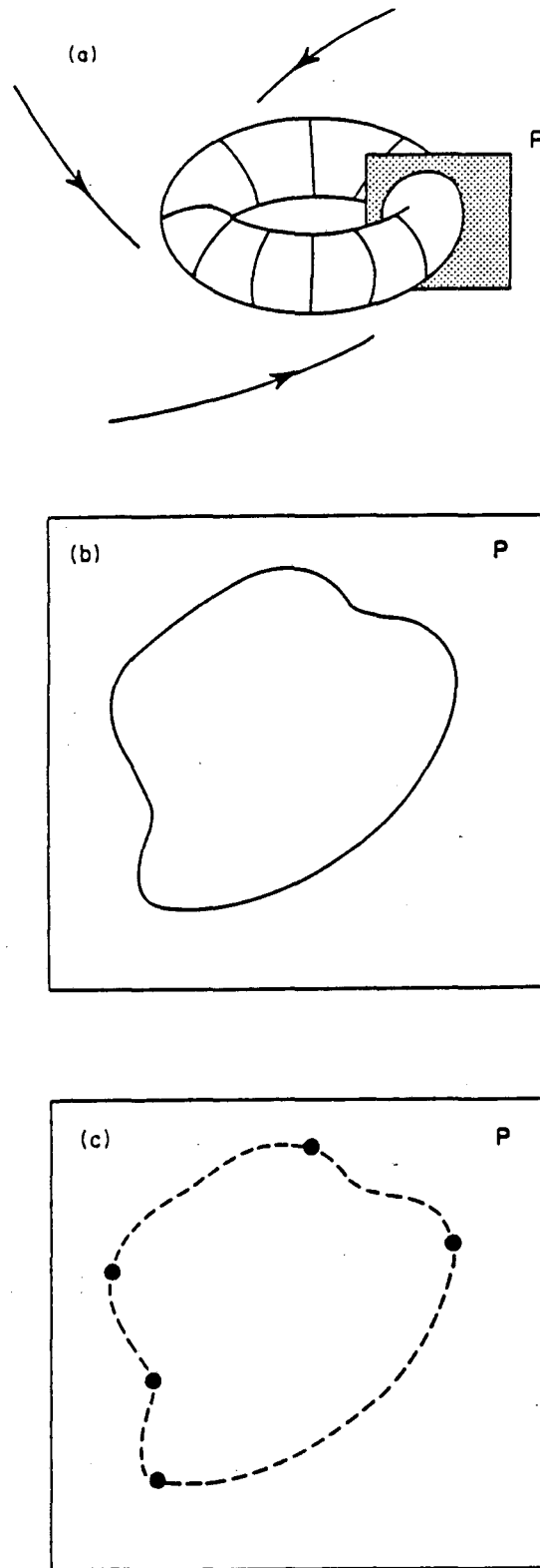
Fig. 5-5: (a) Phase space attraction toward an invariant 2-torus; the Poincaré section P induces an iterative map on the circle. (b) Quasiperiodic dynamics fills in an invariant curve (topologically equivalent to a circle) on P (c) An example of period 5 locked dynamics on P . (from K. Wiesenfeld and I. Satija, Phys. Rev. B 36, 2483 (1987))
