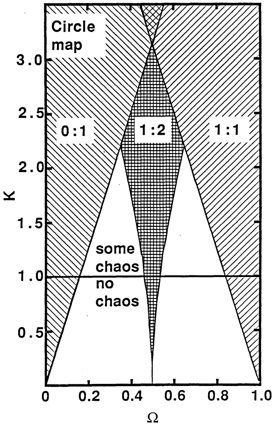
Fig. 7-15- 0:1, 1:2 and 1:1 mode-locked regions for the sine circle map (After Refs. 18,19,35,40). Period doubling and chaos are observed only above the solid line.
