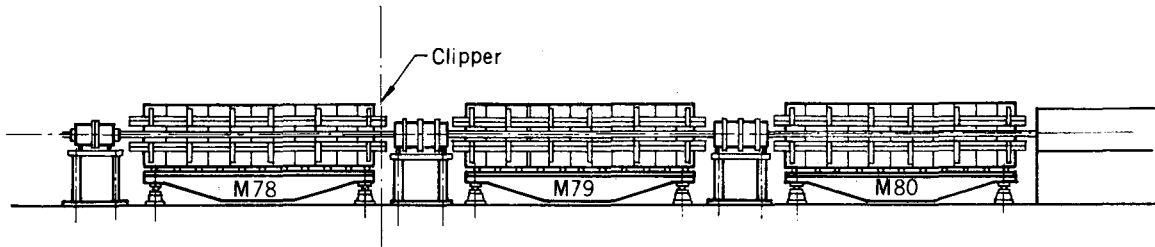
Fig. II-9. Clipper-region target geometry.
