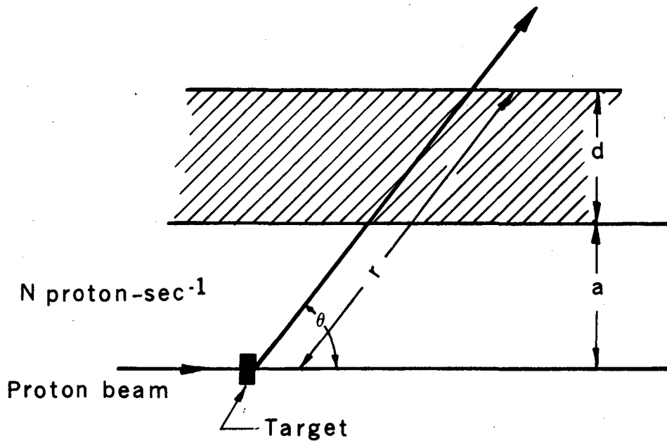
Fig. VIII-1. Schematic representation of typical accelerator geometry.
