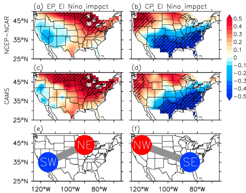
Figure 1. Observed US winter (January–February–March) surface air temperature anomalies regressed onto the (left) EP and (right) CP El Niño indices. Observations correspond to (a, b) the NCEP-NCAR reanalysis and (c, d) the CAMS air temperature data set. Regression coefficients significant at the 90% confidence level based on the student-t test are shaded. (e, f) Schematic diagrams of the EP and CP El Niño impacts on US winter surface air temperatures are also shown.
