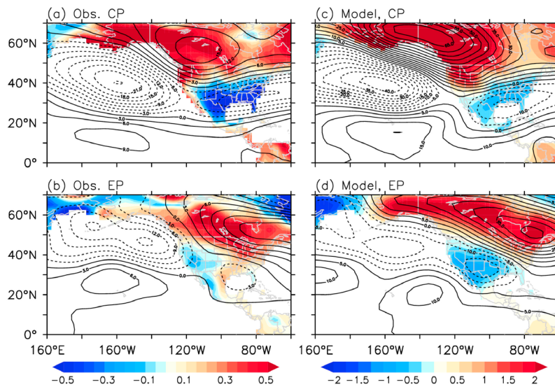
Figure 5. Observed anomalies of 500 mb geopotential heights (contours) and surface air temperatures (color shade) regressed with the (a) CP and (b) EP indices, and the JFM-averaged near-surface air temperature and 500 mb geopotential height differences (c) between the ensemble means of the CP run and the control run and (d) between the ensemble mean of the EP run and that of the control run.
