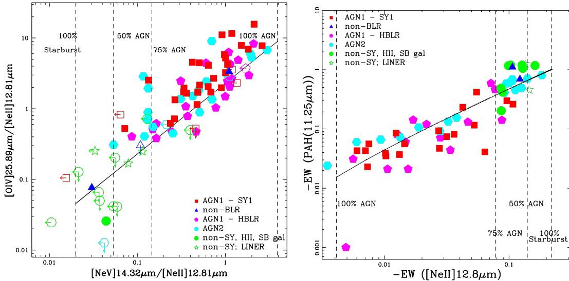
Figure 3. Left panel: [\text{NeV}]14.3\mu\text{m}/[\text{NeII}]12.8\mu\text{m} line ratio versus [\text{OIV}]25.9\mu\text{m}/[\text{NeII}]12.8\mu\text{m} line ratio. Both axes correlate with the strength of the AGN. The black line shows the behaviour of the analytical model (Tommasin et al. 2010). Right panel: [\text{NeII}]12.8\mu\text{m} equivalent width versus PAH 11.25\mu\text{m} equivalent width. Both quantities in this plot correlate with the strength of the star-formation component in each galaxy. The black line shows the behaviour of the analytical model (Tommasin et al. 2010).
