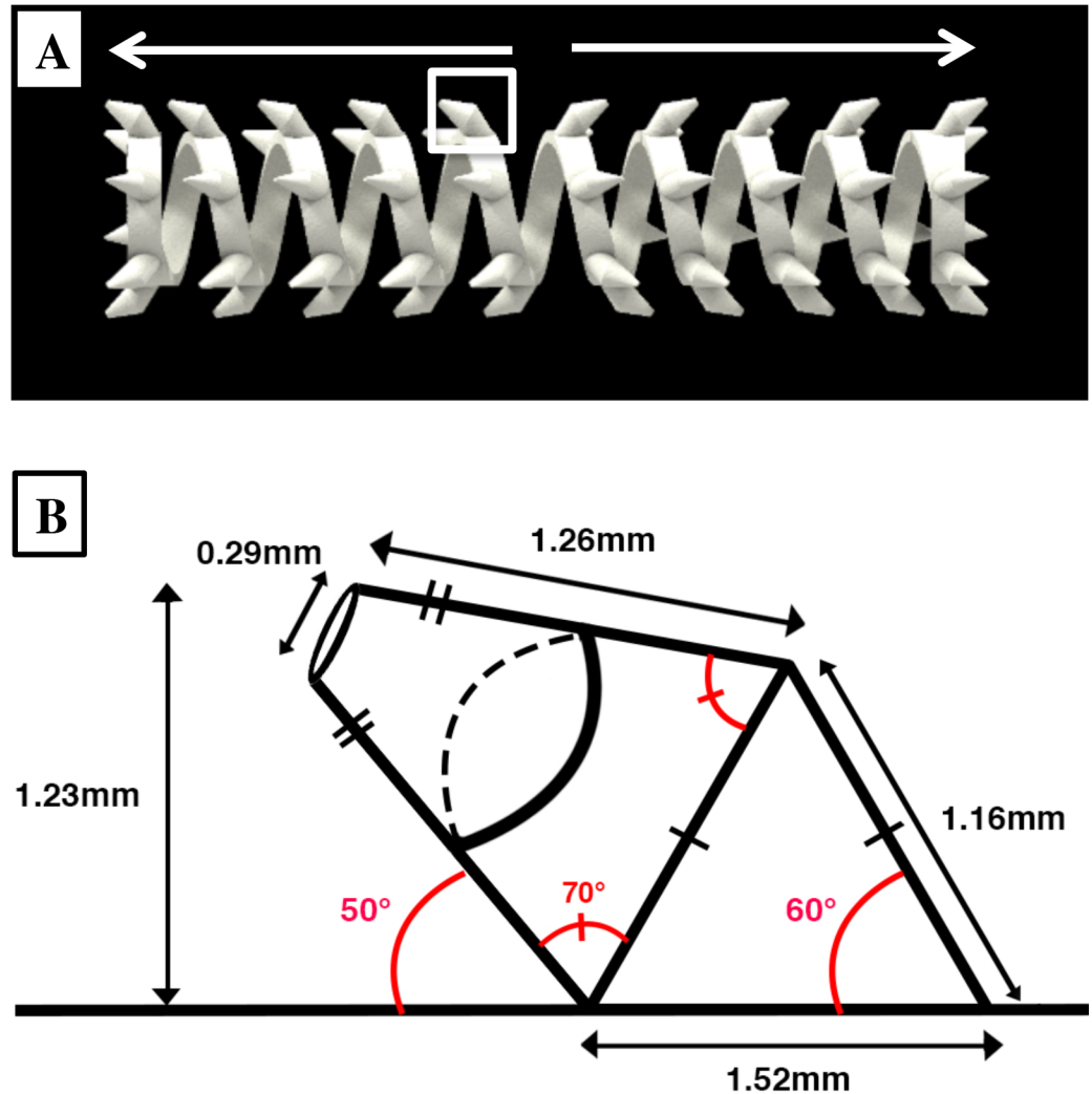
Fig 1. Image of three-dimensionally printed spring with angled bidirectional surface features. (A) Direction of features is indicated by the arrows. One of the surface hooks is isolated by a box. Scale bar is 5 mm. (B) Zoomed in side view schematic of isolated surface feature and corresponding dimensions.
