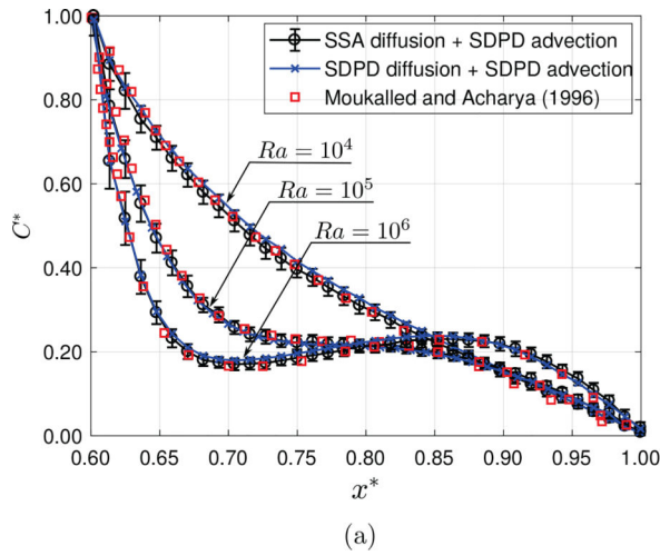
Fig. 5. (a) Comparison of the mean dimensionless concentration ( C^* ) and (b) dimensionless (re-scaled by \sqrt{Ra/Sc} ) y -velocity ( v_y^* ) centerline profiles, for Ra = 10^4 , 10^5 and 10^6 , computed at t = 50 , over Nr = 100 realizations.
