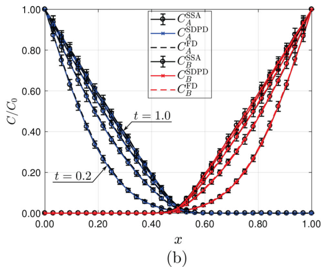
Fig. 3. (a) Schematic of degradation reaction of two arbitrary species, with initial and boundary conditions. (b) Plot of the concentration of the chemical species along the length of the cylindrical domain, at t = 0.2, 0.4, 0.6, 0.8 and 1.0[s] for N = 33 particles.
