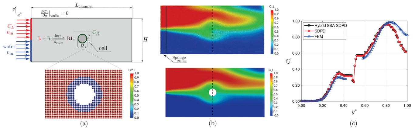
Fig. 6. (a) Upper: schematic of our model of a yeast cell in a microfluidics channel flow containing a pheromone gradient. The working fluid is initially at rest, and at time t > 0 , two inlets start to inject fluid into the chamber; the upper inlet consists of a diluted mixture of working fluid and alpha-factor L , and the lower inlet injects working fluid in the system. (a) Lower: magnified region around the cell, illustrating the particles and their initial velocities. (b) Contour plots of the dimensionless concentration of alpha-factor, C_L^* , at t^* = 2 , obtained using the proposed hybrid method (upper) and FEM (lower). (c) Comparison of the dimensionless concentration profiles of alpha-factor, C_L^* , between hybrid sSSA-SDPD, SDPD and finite element method (FEM), measured across the y^* centerline, at time t^* = 2 . Results shown in (b) were interpolated using a Gaussian kernel, for clarity purposes.
