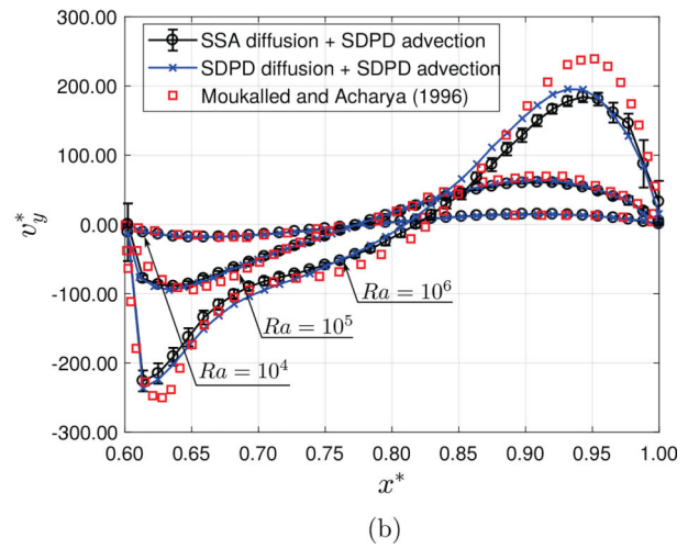
Fig. 5. (a) Comparison of the mean dimensionless concentration ( C^* ) and (b) dimensionless (re-scaled by \sqrt{Ra/Sc} ) y -velocity ( v_y^* ) centerline profiles, for Ra = 10^4 , 10^5 and 10^6 , computed at t = 50 , over Nr = 100 realizations.
