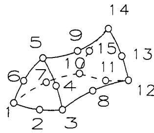
15. PARABOLIC SOLID WEDGE
