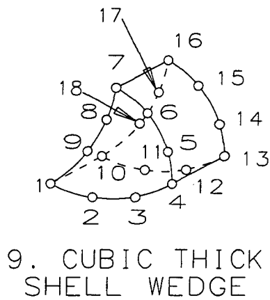
Figure 40. Finite Element Topology Set (continued)
