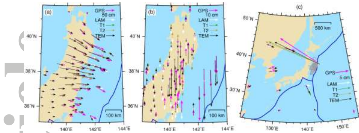
Figure 13. Comparison of two-year postseismic GPS observations at quadtree selected stations with model predicted displacements. (a) Horizontal displacements. (b) Vertical displacements. (c) Comparison of very-far-field GPS observations with model-predicted displacements. Magenta and white arrows represent GPS observations and model-predicted displacements in the LAM, respectively. Structural heterogeneities, the oceanic asthenosphere (OASP), subduction PSP (SPSP), and weakened lower crust beneath the arc (WLCA), are incorporated into the LAM step by step, that is, T1 = \text{LAM} + \text{OASP} , T2 = T1 + \text{SPSP} , and \text{TEM} = T2 + \text{WLCA} .
