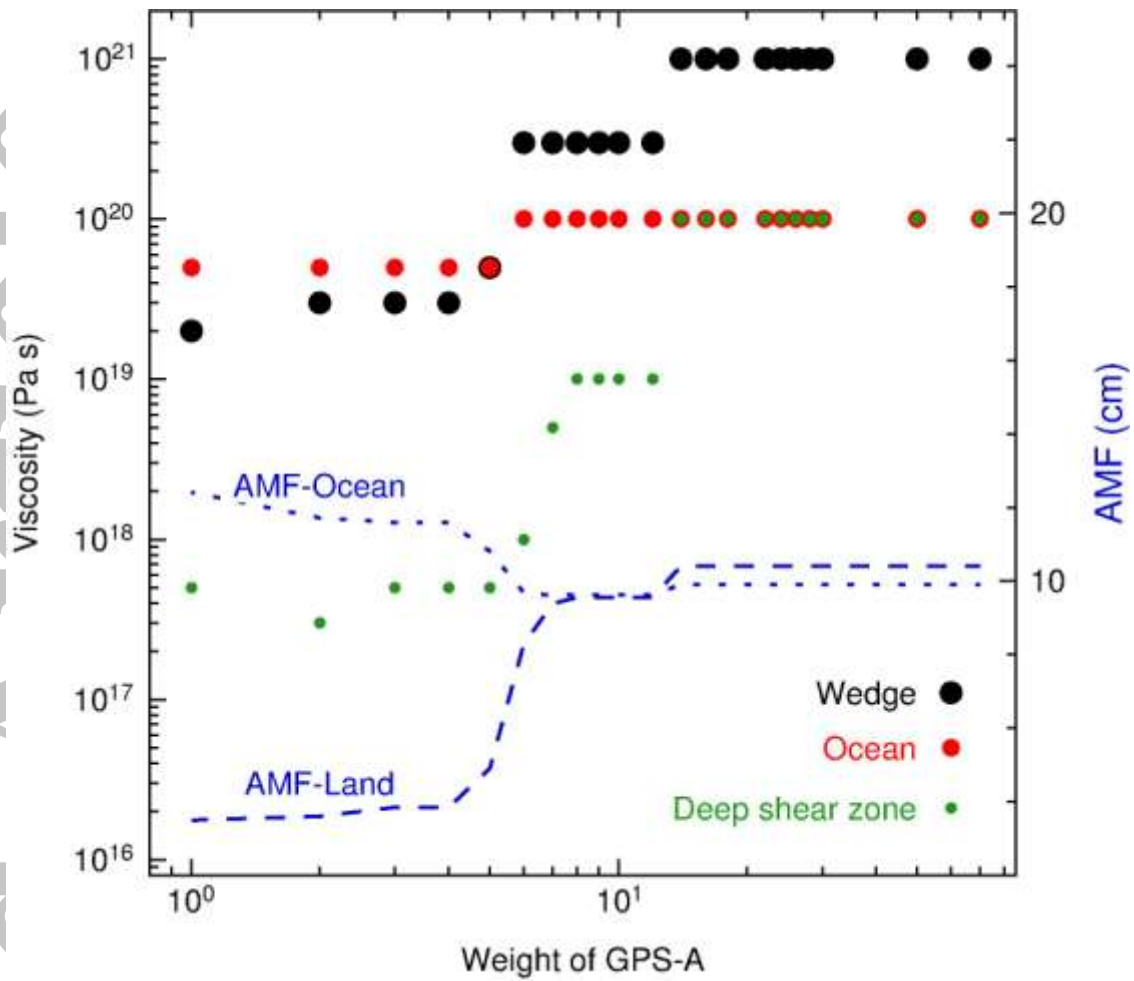
Figure 10. Effects of weights of the GPS-A on the preferred viscosities. Red, black and green symbols are the preferred viscosities of the oceanic upper mantle, mantle wedge, and deep shear zone, respectively at the corresponding weight of the GPS-A. Blue dashed and blue dotted lines represent the AMF of the GEONET (land GPS) and of the GPS-A (offshore) in the corresponding preferred model, respectively.
