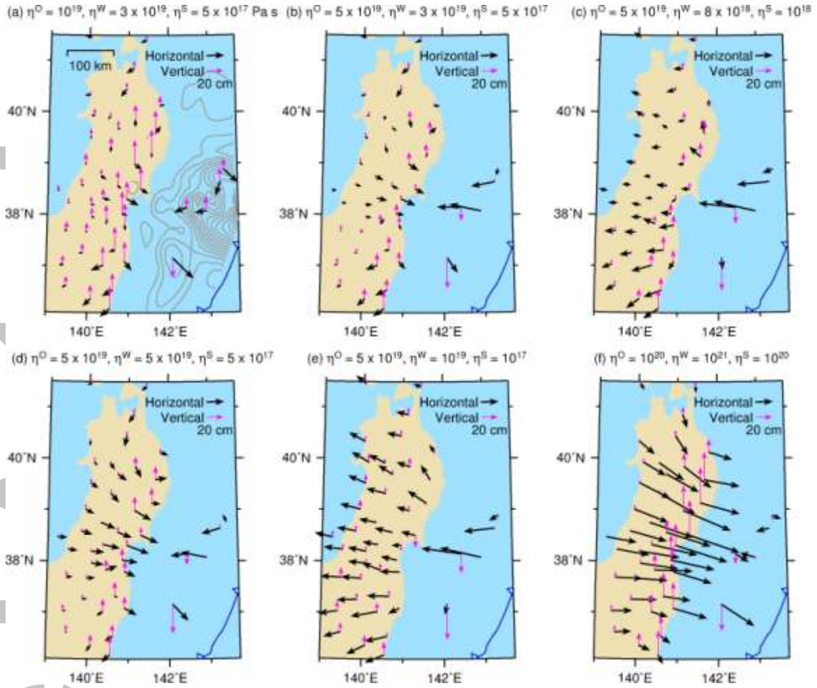
Figure 6. Residuals of two-year postseismic displacements in six test models. Residual is defined as observed displacements at stations selected by the quadtree method (red arrows in Figure 1) minus model-predicted values. Viscosities of each rheological unit of these six models are illustrated in Figures 5d-5f and are also labeled on top of each plot. \eta^O , \eta^W and \eta^S represent steady-state viscosities of the oceanic upper mantle, mantle wedge, and deep shear zone, respectively. Black and magenta arrows represent the horizontal and vertical components, respectively. The test model in (b) is the lowest averaged-misfit model (LAM).
