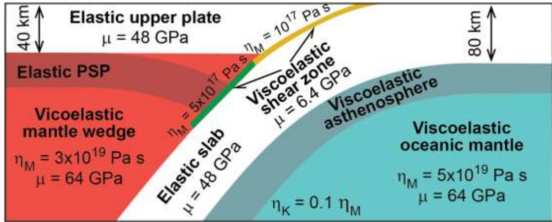
Figure 3. Conceptual representation of the finite element model. The finite element model includes an elastic upper plate and elastic subduction slab (white color blocks), viscoelastic mantle wedge (red), oceanic mantle (cyan) and shear zone along the plate interface (green and brown). Elastic subducting Philippine Sea Plate (PSP) and viscoelastic asthenosphere beneath the oceanic lithosphere (shaded areas, not to scale) will be discussed in Section 5. \mu is the shear modulus. The shown steady-state viscosity values \eta_M are ten times the corresponding transient viscosity \eta_K . The viscosities shown represent the determined values found in the three-parameter optimization described in section 4.2.
