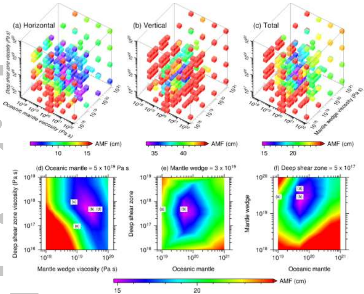
Figure 5. Misfit of test models and trade-off between the upper mantle rheology and deep shear zone rheology. Averaged misfit (AMF, from Equation 1) is calculated from horizontal (a), vertical (b), or both horizontal and vertical displacements (c-f). Trade-offs of model parameters in this work are displayed as the relationship between viscosity-values between any two of the three rheological elements, the oceanic upper mantle, mantle wedge and deep shear zone, while the viscosity of the third is fixed to the LAM value. (d) The viscosity of the oceanic mantle is fixed at 5 \times 10^{19} Pa s, and viscosities of the mantle wedge and deep shear zone are variable. (e) The viscosity of the mantle wedge is fixed at 3 \times 10^{19} Pa s. (f) The viscosity of the deep shear zone is fixed at 5 \times 10^{17} Pa s. Misfits of test models labeled in (d) – (f) are plotted in Figure 6.
