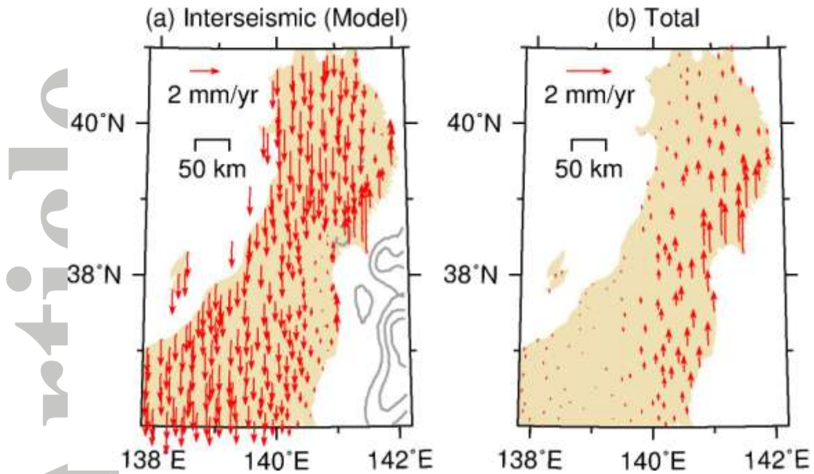
Figure 16. Alternative model-predicted interseismic vertical velocities and the net effects of vertical deformation in earthquake cycles. (a) Modeled interseismic vertical deformation by assuming that the released strain of the 2011 earthquake was accumulated linearly with time in the last 600 years. (b) Total effects of (a) and Figures 15b – 15d.
