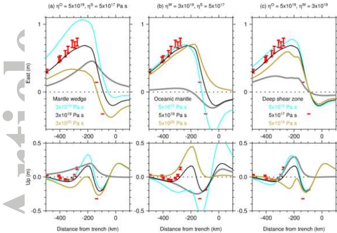
Figure 7. Sensitivities of the surface deformation to the viscosity change in the mantle wedge (a), oceanic upper mantle (b) and deep shear zone (c). Two-year postseismic displacements are plotted along a surface profile at latitude 38°N. Upper and lower panels are East and upward directions, respectively. Red error bars represent observations at GEONET and GPS-A within 20 km of the profile line. In each column, the viscosity of one rheological element is varied while the other two rheological elements are fixed at the same viscosities as in the LAM (labeled at the top). Color-coding of the lines representing models of different viscosities is described in the insert text. Grey lines in (a) and (b) represent the same test models as shown in Figures 4a – 4b in which the viscosity of one rheological unit is at the same value as in the LAM (black color) while the other two rheological elements are assumed to be ELASTIC (infinite viscosity). Grey lines in (c) are the combined effects of Figures 4c and 4d. Black lines are the same LAM in all three columns.
