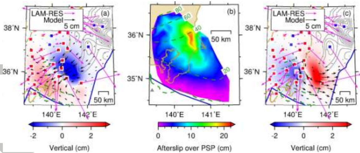
Figure 12. Effects of the elastic subducting Philippine Sea plate (PSP) and afterslip on the PSP-OKT plate interface on the surface deformation. (a) Surface displacements two years after the earthquake only due to the elastic PSP slab. Similar to Figure 11, black arrows and color contours represent horizontal and vertical model displacement components, respectively. Magenta arrows and filled white squares represent the spatially down-sampled horizontal and vertical residuals of GPS observations in the LAM as shown in Figure 8. Thick green dashed lines represent the depth contours (labeled in (b)) of the top of the PSP slab (Uchida et al. , 2010b). Thick blue solid lines represent the location of the trench. (b) Modeled amplitude of afterslip on the PSP-OKT plate boundary with a viscosity 10^{19} Pa s in the shear zone. (c) Surface deformation in the first two years after the earthquake only due to the PSP-OKT afterslip shown in (b).
