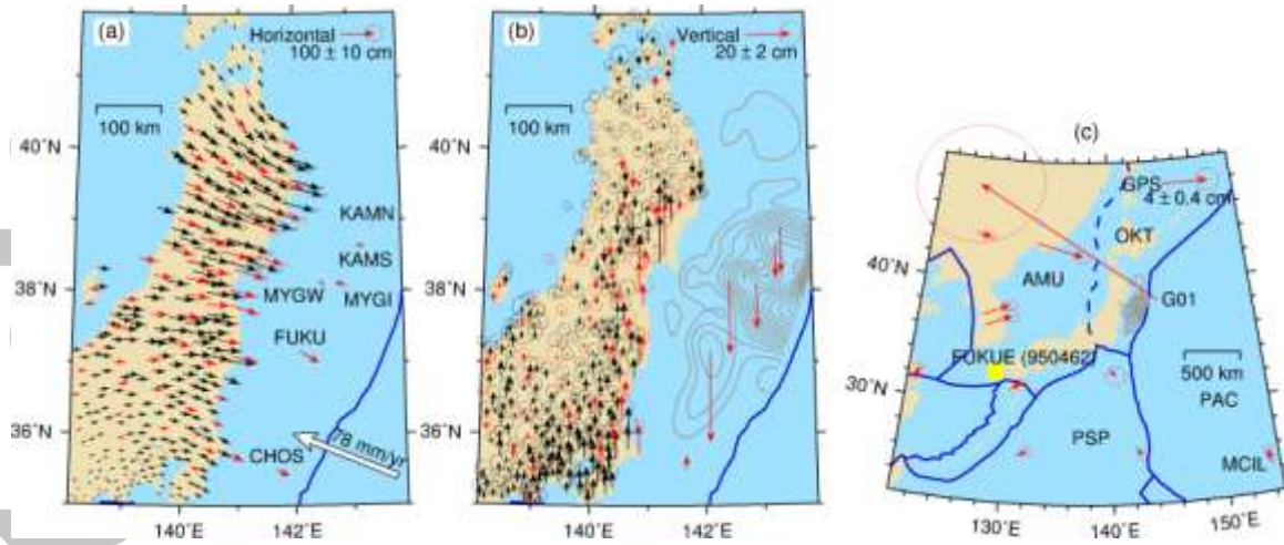
Figure 1. Postseismic GPS observations in the first two years following the 2011 Tohoku earthquake. Horizontal (a) and vertical (b) GPS displacements of GEONET and GPS-A stations. Red arrows represent the GPS stations selected to evaluate test models through quadtree method (see text for details). Black arrows are those not selected. (c) Horizontal postseismic GPS observations of five far-field IGS stations, one GPS-A station G01 and far-field GEONET stations in the Philippine Sea and Pacific plates. Displacements of G01 are averaged from 09/11/2012 to 10/17/2014 (Tomita et al. , 2015). Grey contours in (b) and (c) are the coseismic rupture of the 2011 Tohoku earthquake at intervals of 5 m (Inuma et al. , 2012). All the GPS displacements are corrected for interseismic deformation and are referenced to station FUKUE (ID 950462) whose location is shown by a solid yellow square in (c). PAC, OKT, AMU and PSP denote the Pacific, Okhotsk, Amuria, and Philippine Sea plates.
