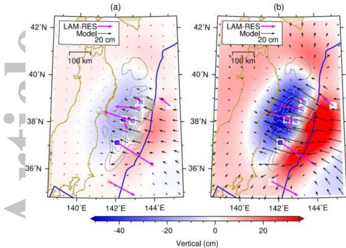
Figure 11. Effects of the viscoelastic relaxation in an 80-km-thick weak asthenosphere beneath the oceanic lithosphere on the surface deformation. Black arrows and color contours represent modeled horizontal and vertical surface postseismic deformation in the first two years after the earthquake, respectively. Magenta arrows and filled white rectangles represent the horizontal and vertical residuals of GPS-A stations in the LAM as shown in Figure 8. The color scale of the vertical components of the misfit and model predictions is the same. The viscosity of the asthenosphere is 10^{19} Pa s in (a) and 10^{18} Pa s in (b). The viscosity of the oceanic upper mantle is 5 \times 10^{19} Pa s in (a) and 10^{20} Pa s in (b).
