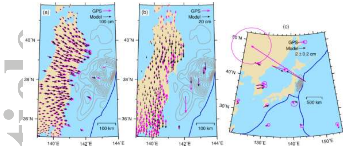
Figure 8. Comparison of GPS observations with the LAM two years after the 2011 earthquake. Magenta and black arrows represent GPS observations and model-predicted displacements, respectively. (a) Horizontal displacements. (b) Vertical displacements. (c) Comparison of very-far-field GPS observations with model-predicted displacements.
