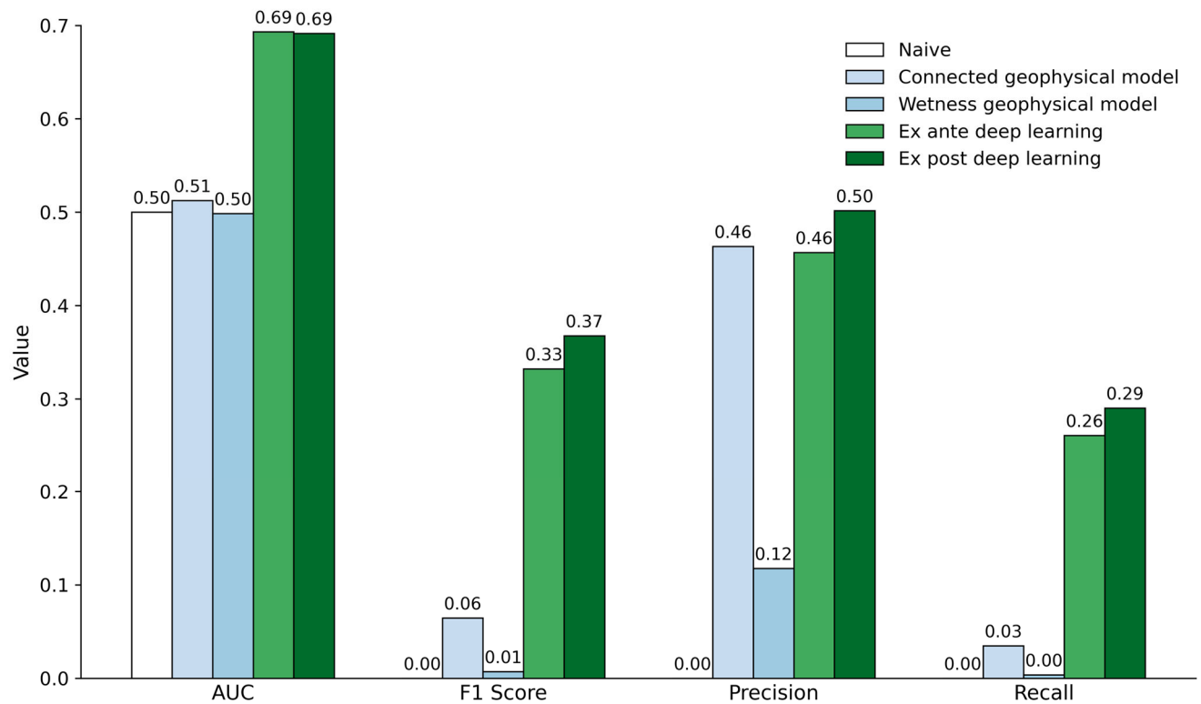
Fig. 1: Geophysical models have similar or somewhat better performance than the naïve benchmark, ex ante deep learning does much better, and ex post deep learning has the strongest model performance.
