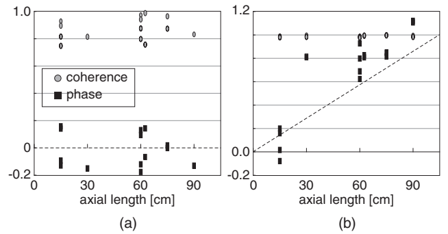
Fig. 7. Results from axial correlation analysis at r = 4 cm. Squared cross-coherence and cross-phase ( \text{rad}/2\pi ) of the (a) ZF and (b) DW. Dashed lines indicate n = 0 (a) and 2 (b), where n = 1 shows that axial wavelength is the same as vessel length. The significance level is 0.0625 .
