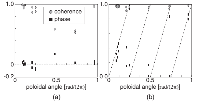
Fig. 6. Results from poloidal correlation analysis measured at r = 4 cm. Squared cross-coherence and cross-phase ( \text{rad}/2\pi ) of the (a) ZF and (b) DW. Dashed lines indicate m = 0 (a) and 4 (b). The significance level is 0.0625 .
