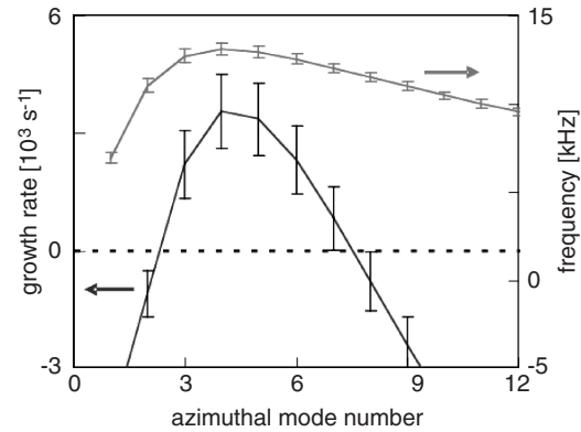
Fig. 10. Results from numerical linear device code. Growth rates and real frequencies versus azimuthal mode number are shown. Fluctuations with m = 3-7 are unstable.
