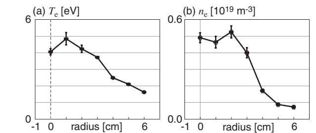
Fig. 5. Equilibrium radial profiles of the (a) electron temperature T_e (eV) and (b) electron density n_e ( 10^{19} \text{ m}^{-3} ).
