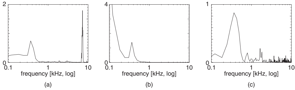
Fig. 11. Amplitude modulation of the DW synchronized at the ZF oscillation measured at r = 3.25\text{--}3.5 cm (SN 5716, 0.1–0.37 s average). (a) Auto-power of original \Phi_f , (b) auto-power of the envelope of \Phi_f in 6.5–7.5 kHz frequency range. A linear scale is chosen in the vertical axis. (c) Squared cross-coherence between original and envelope waves.
