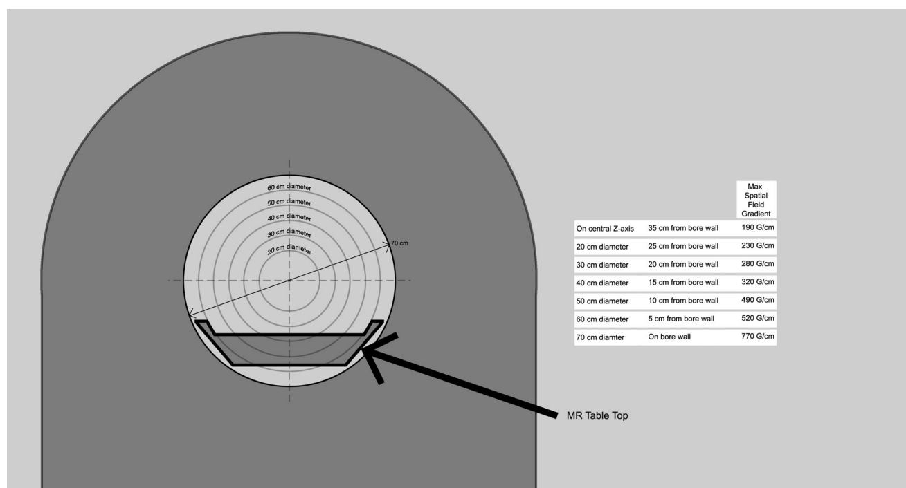
FIGURE 1: Axial view SFG map of an MR system indicating maximum SFG values that may be encountered within each of the nested cylindrical volumes within the diameter of the bore. Illustration courtesy of Tobias Gilk.
