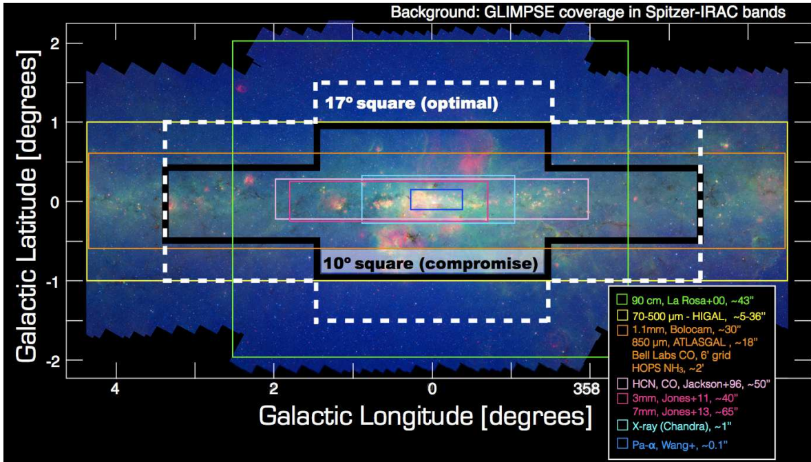
Fig. 3.— Recommended coverage areas for a deep VLASS mosaic of the Galactic center in C band (4-8 GHz) continuum, recombination lines, \text{H}_2\text{CO} , and \text{CH}_3\text{OH} masers, compared to coverage of existing surveys. The diffuse red emission at l = 359.5, b = 0.5 enclosed in a shell of green emission is the GC lobe (Sofue 1985), suggested to be an outflow from the Galaxy’s nucleus.
