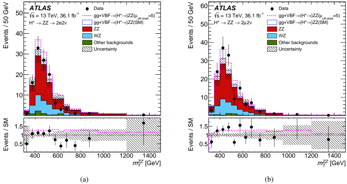
Figure 2: Observed transverse mass m_{\text{T}}^{ZZ} distribution in the (a) ee channel and (b) \mu\mu channel of the ZZ \rightarrow 2\ell 2\nu off-shell region, compared to the expected contributions from the SM including the Higgs boson (stacked). Events with 1500 < m_{\text{T}}^{ZZ} < 2000 GeV are included in the last bin of the distribution. The hatched area shows the combined statistical and systematic uncertainties. The dashed line corresponds to the total expected event yield, including all backgrounds and the Higgs boson with \mu_{\text{off-shell}} = 5 . The ratio plot shows the observed data yield divided by the SM prediction (black points) as well as the total expected event yield with \mu_{\text{off-shell}} = 5 divided by the SM prediction (dashed line) in each bin.
