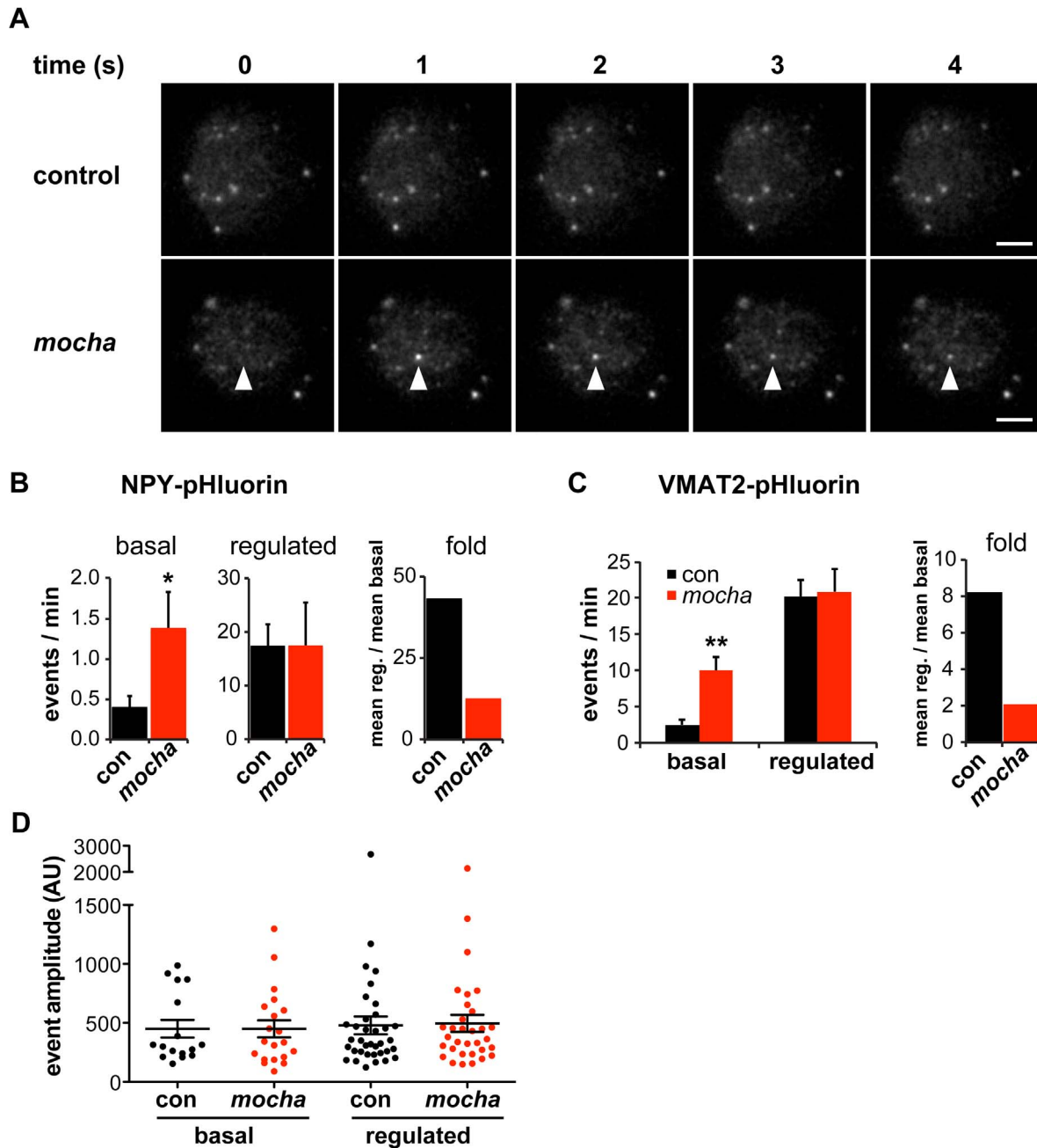
Figure 1. mocha chromaffin cells display dysregulated release of NPY and VMAT2. Chromaffin cells were transduced with lentivirus encoding either NPY- or VMAT2-pHluorin, then imaged live 4–7 days later by TIRF microscopy. Basal exocytosis was measured in Tyrode's solution, and release stimulated in Tyrode's containing 5 \mu M DMPP. (A) Representative images acquired during the unstimulated phase show a typical basal exocytotic event in a mocha cell. Scale bars indicate 5 \mu m. (B) Quantification of individual exocytotic events shows increased basal NPY-pHluorin exocytosis in mocha cells, and a similar number of events relative to control cells after stimulation. * p < 0.04 relative to control; for basal, n = 38 for control and n = 38 for mocha ; for stimulated, n = 22 for control and n = 22 for mocha . Normalizing mean regulated events to mean basal events shows that mocha cells have an \sim 70\% reduction in secretion fold change in response to stimulation relative to control cells. (C) Quantification of exocytotic events as above shows increased basal VMAT2-pHluorin exocytosis in mocha cells. ** p < 0.0003 relative to control; n = 18 for control and n = 16 for mocha . Analysis of the secretion fold change shows that mocha cells have an \sim 75\% reduction relative to control. (D) Analysis of the amplitude of exocytotic events monitored using NPY-pHluorin reveals that basal and regulated events of both control and mocha cells are comparable in size. The bars indicate mean values, and error bars the s.e.m. doi:10.1371/journal.pgen.1003812.g001
