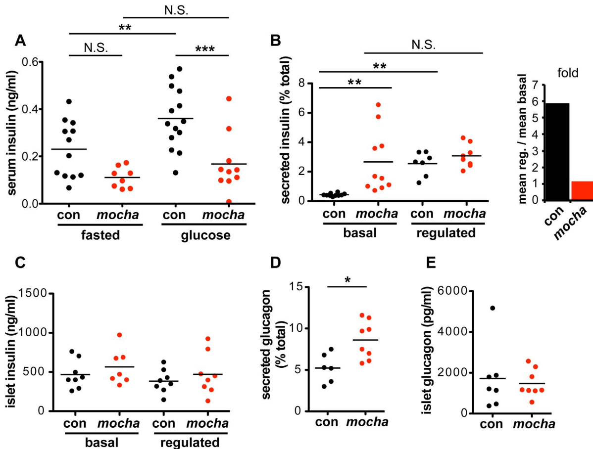
Figure 2. mocha mice show dysregulated secretion of insulin and glucagon. (A) Serum insulin levels were determined after an overnight fast (baseline) and 15–20 min after i.p. injection of glucose (2 mg/g body weight). In contrast to the controls, mocha insulin levels do not significantly increase after glucose injection. The data derive from two independent experiments; n = 14 control and n = 10 mocha mice. ** p < 0.01 ; *** p < 0.001 by Newman-Keuls post-hoc test. Pancreatic islets were isolated acutely and bathed in either 2.8 mM (basal) or 28 mM (regulated) glucose for 1 h at 37°C. (B) mocha islets display markedly increased basal insulin secretion compared to controls. In contrast, control and mocha islets secrete comparable amounts of insulin in response to high glucose. For control islets, this represents an ~6-fold increase in secretion in response to glucose elevation. For mocha islets, insulin secretion is not significantly increased in response to glucose elevation. ** p < 0.01 by Dunnett's post-hoc test, n = 7 –10. (C) After collecting secreted insulin, the islets were pelleted and lysed by sonication to extract cellular insulin. Cellular insulin levels are similar between all groups. (D) Basal glucagon secretion measured in 28 mM glucose is significantly increased by the mocha mutation. (E) Cellular glucagon levels do not differ between mocha and control mice. * p < 0.02 , n = 6 –8. The bars represent mean values. doi:10.1371/journal.pgen.1003812.g002
