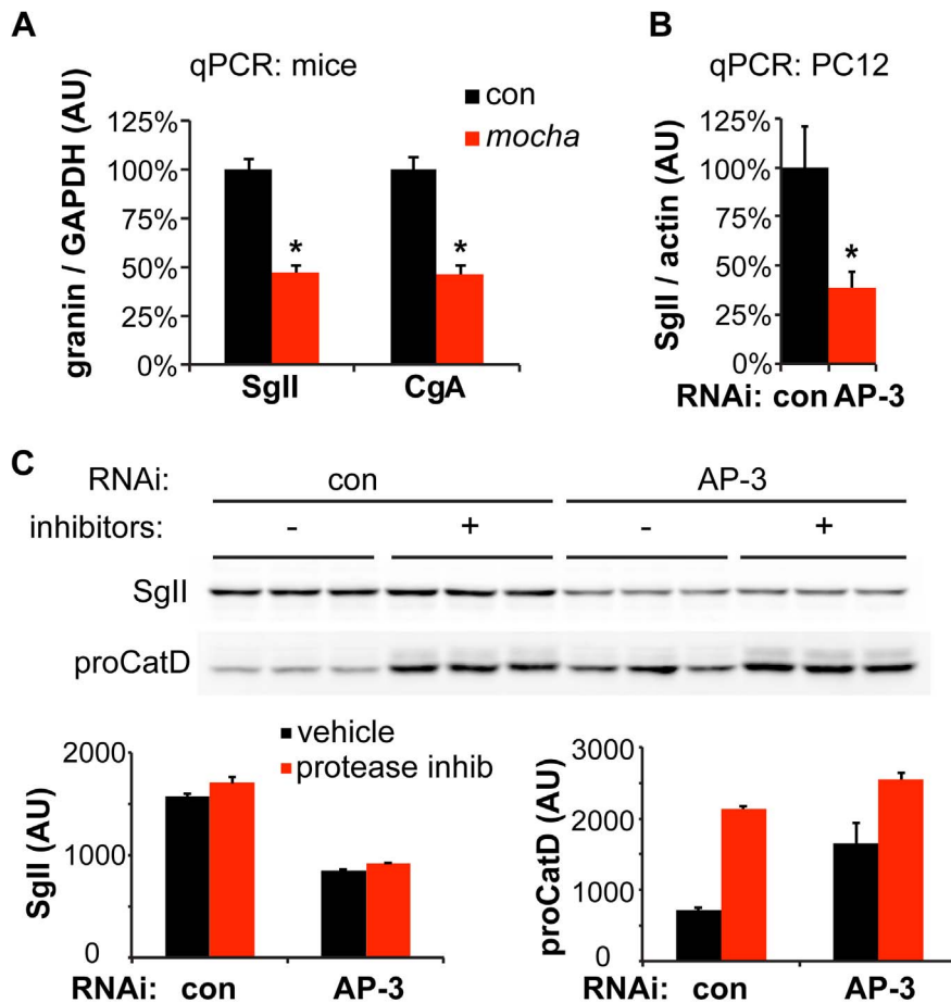
Figure 4. Loss of AP-3 reduces granin mRNA but does not increase its degradation. (A) Quantitative RT-PCR (qPCR) analysis of adrenal gland transcripts from mocha mice shows an ~50% reduction in SgII and CgA expression relative to the adrenals of littermate controls. *p < 1 \times 10^{-4} , n = 6-7 adrenals per genotype. (B) qPCR analysis of PC12 cells transfected with AP-3 \delta siRNA shows an ~60% reduction in SgII expression relative to cells transfected with control siRNA. *p < 0.02 , n = 5-6 transfections. (C) Incubation of PC12 cells with lysosomal protease inhibitors for ~24 h has no effect on cellular SgII levels in cells transfected with either AP-3 \delta or control siRNA. In contrast, the protease inhibitors markedly elevate the levels of the lysosomal hydrolase precursor procathepsin D. The data show mean values, and error bars indicate s.e.m. doi:10.1371/journal.pgen.1003812.g004
