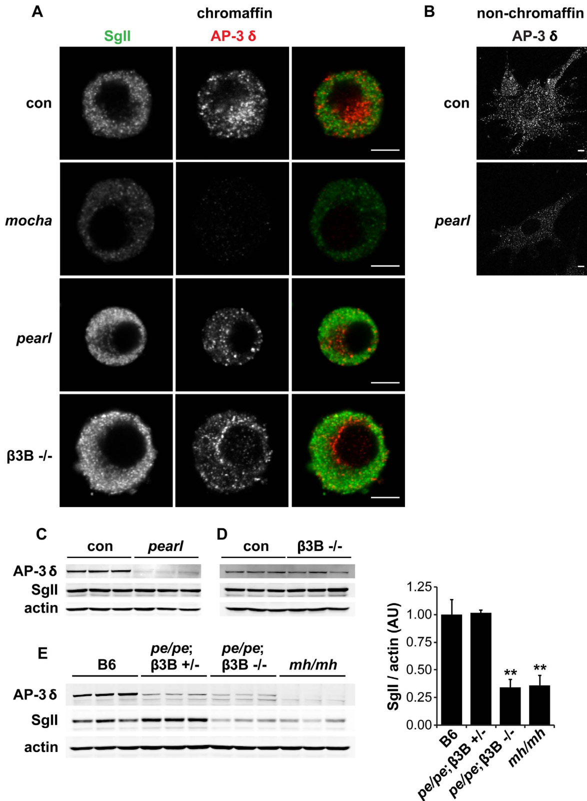
Figure 3. Concomitant loss of both \beta 3A and \beta 3B is required to reduce adrenal SgII. (A) Effect of individual AP-3 subunit mutations on SgII and AP-3 \delta levels by immunofluorescence. Adrenal chromaffin cells from mocha ( \delta ), pearl ( \beta 3A ), \beta 3B^{-/-} , and control mice were stained with a rabbit polyclonal antibody to SgII and a mouse monoclonal antibody to AP-3 \delta , followed by an anti-rabbit antibody conjugated to Alexa Fluor 488 and an anti-mouse antibody conjugated to Alexa Fluor 594. Representative confocal micrographs show the expected reduction in SgII and absence of AP-3 \delta staining in mocha chromaffin cells, but unchanged SgII and AP-3 \delta in both pearl and \beta 3B^{-/-} cells. (B) Non-chromaffin, fibroblast-like pearl cells present in the culture show a clear reduction in AP-3 \delta . Scale bars indicate 5 \mu m . (C) The adrenal glands of pearl mice show a clear reduction in overall
