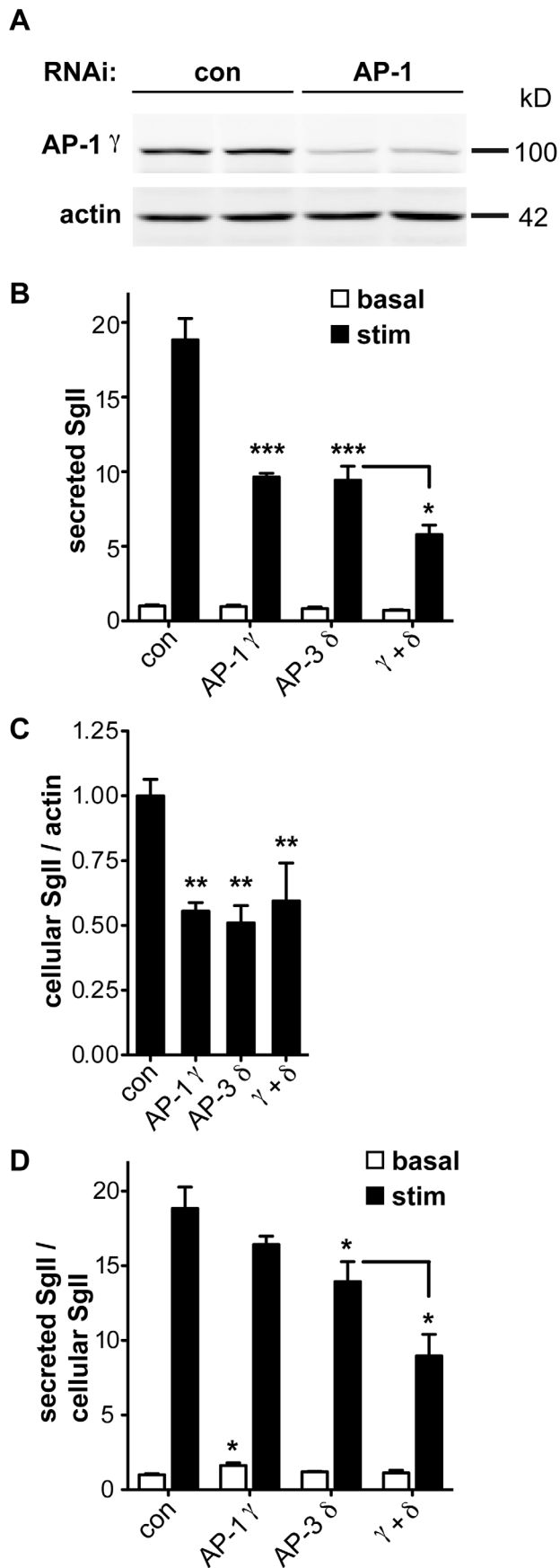
Figure 5. AP-1 knockdown potentiates the effect of AP-3 knockdown on regulated secretion. (A) PC12 cells were transfected with pooled siRNA directed against AP-1 \gamma or pooled nontargeting siRNA as control. Knockdown was assessed by quantitative fluorescent immunoblotting for AP-1 \gamma with actin as loading control. (B) PC12 cells were transfected with control, AP-1 \gamma , AP-3 \delta or both siRNAs, washed, and incubated for 30 min in Tyrode's solution containing 2.5 mM (basal) or 50 mM (stimulated) K^+ . Secreted SgII was measured by quantitative fluorescent immunoblotting and normalized to basal secretion from cells treated with control siRNA. AP-1 \gamma RNAi alone reduces the depolarization-induced secretion of SgII very similar to AP-3 \delta RNAi, and combined AP-1 \gamma /AP-3 \delta RNAi potentiates the decrease in regulated secretion. (C) Cells were lysed and intracellular SgII measured as above, normalizing to actin. AP-1 \gamma and AP-3 \delta RNAi both reduce cellular SgII, but the combined knockdown does not show an additional effect. (D) Secreted SgII was normalized to cellular SgII levels for each RNAi condition, and expressed relative to basal secretion from cells treated with control siRNA. Normalizing to cellular SgII shows a significant increase in basal secretion of SgII with AP-1 \gamma RNAi whereas AP-3 \delta RNAi significantly reduces depolarization-induced secretion. Combined AP-1 \gamma /AP-3 \delta RNAi potentiates the reduction in stimulated release. * p < 0.05 ; ** p < 0.01 ; *** p < 0.001 (Newman-Keuls post-hoc test; n = 4 transfections). The data show mean values, and error bars indicate s.e.m.
