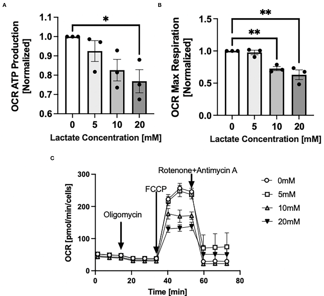
FIGURE 5 | Mitochondrial oxygen consumption rate with chronic lactate treatment. NRVMs were treated for 48 h with various concentrations of lactate and oxygen consumption rate assessed using the Seahorse analyzer. (A) Rate of ATP production normalized to untreated cells (untreated range 8.5 to 16.3 pmol/min/cell), (B) Rate of maximal respiration normalized to untreated cells (untreated range 132.5 to 386.4 pmol/min/cell). (C) Seahorse trace for a representative NRVM preparation day. n = average of 3 cell preparations; error bars show standard error of the mean, * p < 0.05, ** p < 0.01.
