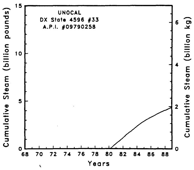
Figure A-50 Steam rate and cumulative mass flow for well DX State 4596 #33
