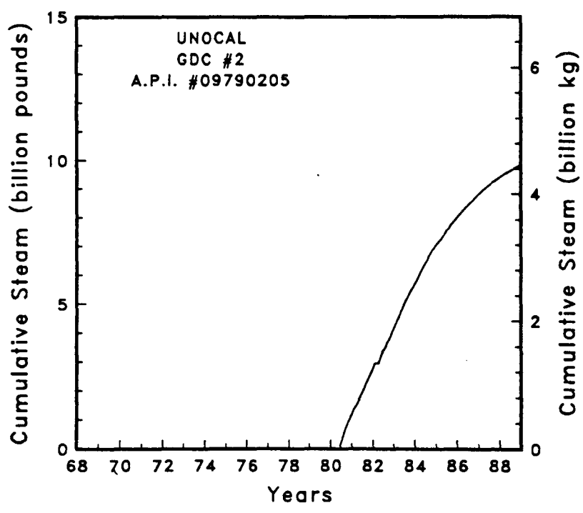
Figure A-76 Steam rate and cumulative mass flow for well GDC #2
