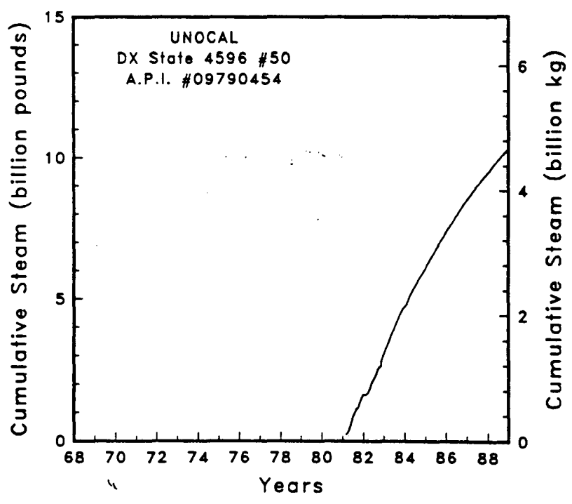
Figure A-61 Steam rate and cumulative mass flow for well DX State 4596 #50
