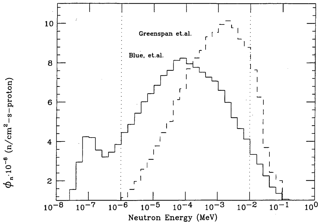
Figure 13: Neutron spectral shape for assembly designs #1 (BeO moderator by Blue) and #3 ( {}^7\text{Li}/\text{Pb} by Greenspan). The \Phi_n is identical in both cases and is equal to 1.3 \times 10^{-4} (n/cm 2 -s-proton). Both spectrums are produced from incident 2.5 MeV proton beams.
