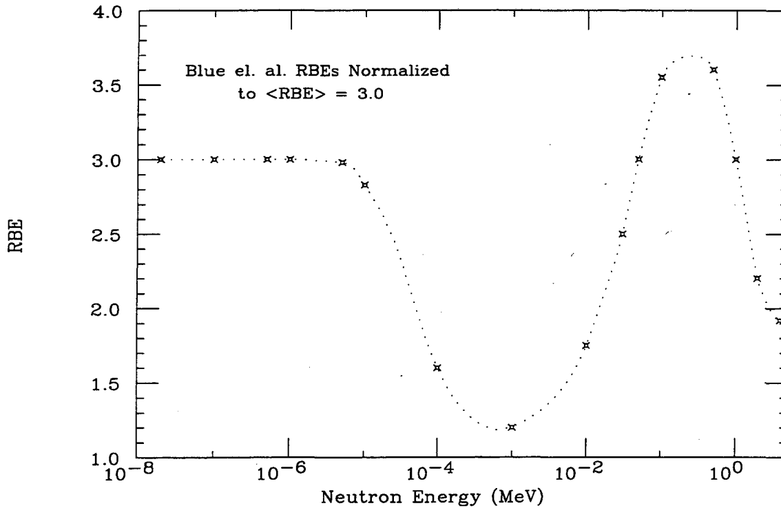
Figure 5: Neutron energy dependent RBE from Blue (REF) normalized to produce an energy-averaged RBE of 3.
