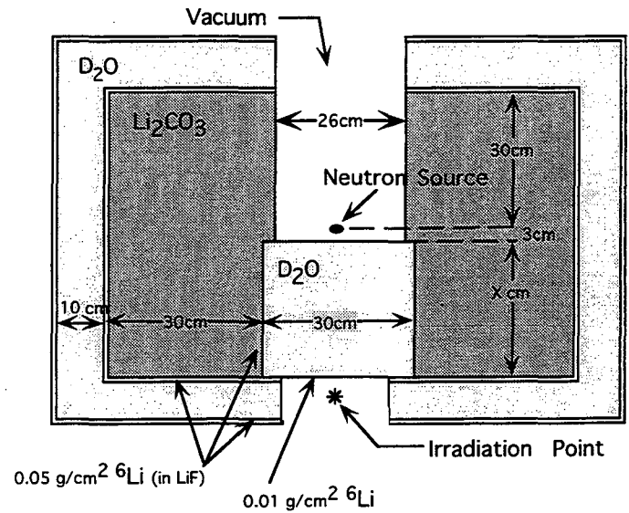
Assembly Design #4 (Blue et. al.)
