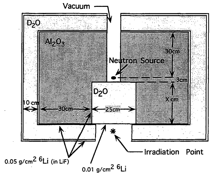
Assembly Design #2 (Blue et. al.)
