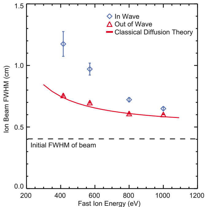
FIG. 8. (Color online) Beam FWHM vs energy with the plate inserted (diamond) and retracted (triangle). The solid line shows the dependence predicted by classical diffusion theory. The dashed line is the initial beam width caused by the finite aperture size of the ion source.
