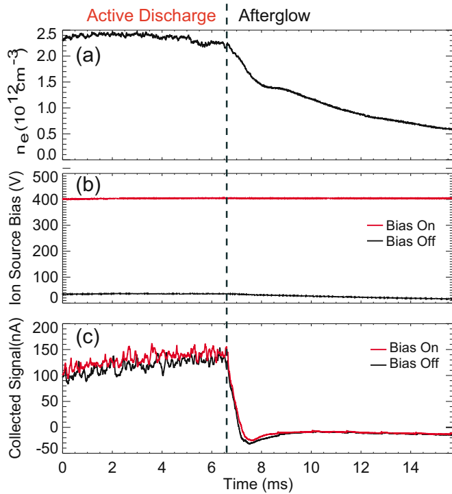
FIG. 3. (Color online) Typical time evolution of (a) plasma density, (b) ion source operating voltage, and (c) collected signal during the data collection time window. The active discharge ends at \sim 6.5 ms. (a) Line-averaged plasma density measured by the interferometer. (b) Operating voltage on the ion source to launch a 400 eV ion beam. (c) Collected signal when the ion source operating voltage is on/off. The fast ion signal is the difference between these two. Signal collected three ports from the source.
