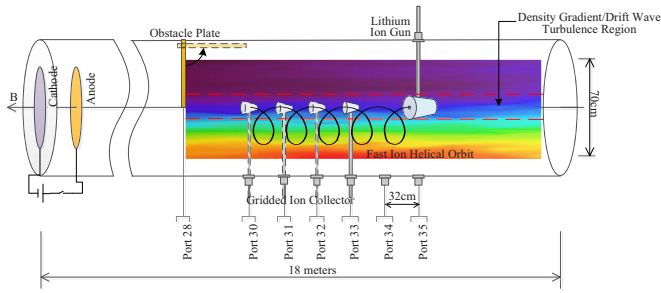
FIG. 1. (Color online) Experimental setup in the LAPD. Fast ions interact with drift wave turbulence in the region between the two dash lines. The probe is inserted at different ports each time to study the spatial dependence of transport. The ion source and analyzer are axially aligned. The contour shows a typical density profile when plate-obstacle is deployed.
