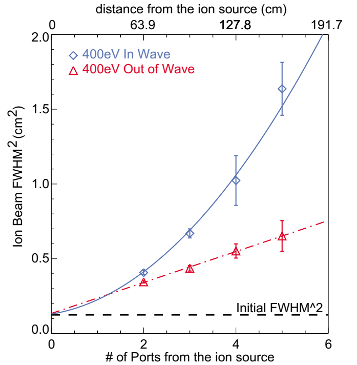
FIG. 10. (Color online) The square of the radial ion beam FWHM vs distance from the source. The out of wave data are fitted by a linear function. The in wave data are fitted by a polynomial function of second order.
