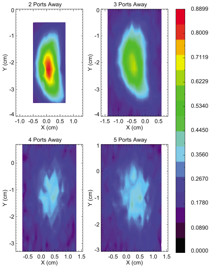
FIG. 9. (Color online) Beam profile collected at different distances away (2–5 ports/31.95–159.75 cm) from the ion source.
