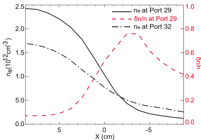
FIG. 2. (Color online) Horizontal profiles of density at two different axial positions (solid and dash-dot lines) and of density fluctuations (dashed line), averaged between 2–6.5 ms in the active discharge. The edge of the plate-obstacle is at x = 0 , and the ionizing fast electrons are blocked in the x > 0 region.
