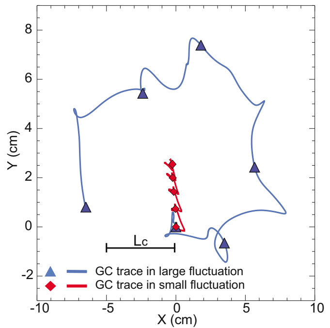
FIG. 15. (Color online) The trajectory of an individual guiding center in a representative turbulent potential structure. The triangles and diamonds show the fast ion GC position after each cyclotron orbit, 0–5 ports away from the ion source for turbulence with large triangle and small diamond amplitude.
