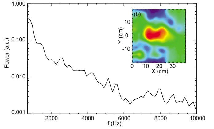
FIG. 13. (Color online) The characteristics of drift wave turbulence simulated by the BOUT code. (a) Fluctuation power spectrum. (b) Cross-correlation of the potential fluctuation.
