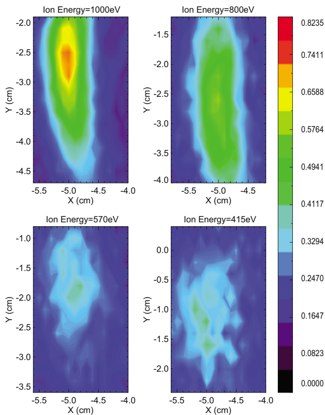
FIG. 7. (Color online) Typical beam profiles for different fast ion energies, collected three ports (95.85 cm) away from the ion source.
