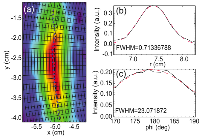
FIG. 6. (Color online) A typical collected beam profile and data analysis process. (a) Contour of the signal amplitude. Dotted line: fitted gyro-orbit. Solid line: mesh imposed to calculate the beam FWHM. (b) Beam radial profile and its gauss fit. (c) Beam azimuthal profile and its gauss fit.
