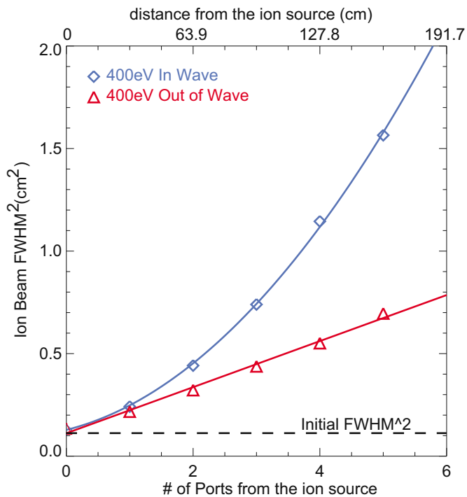
FIG. 14. (Color online) Monte-Carlo simulated fast ion FWHM (Ref. 2) as a function of distance (time). Triangles denote the effect of the classical transport, and is fitted by a linear function. Diamonds denote the effect of both turbulent wave and classical transport, and is fitted by a polynomial function of second order.
