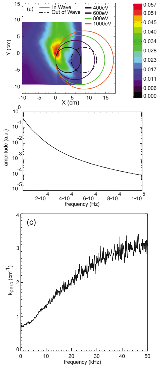
FIG. 4. (Color online) Characteristics of drift wave turbulence created by the plate-obstacle. (a) Contour of the total power of the wave with frequency ranges of 0.7–100 kHz, fast ion orbits with different energies is overlaid to show the overlap between the waves and particles. (b) Averaged fluctuation power spectrum (log-log). (c) Dispersion relation of the wave, calculated from the cross-correlation between two triple probes.
