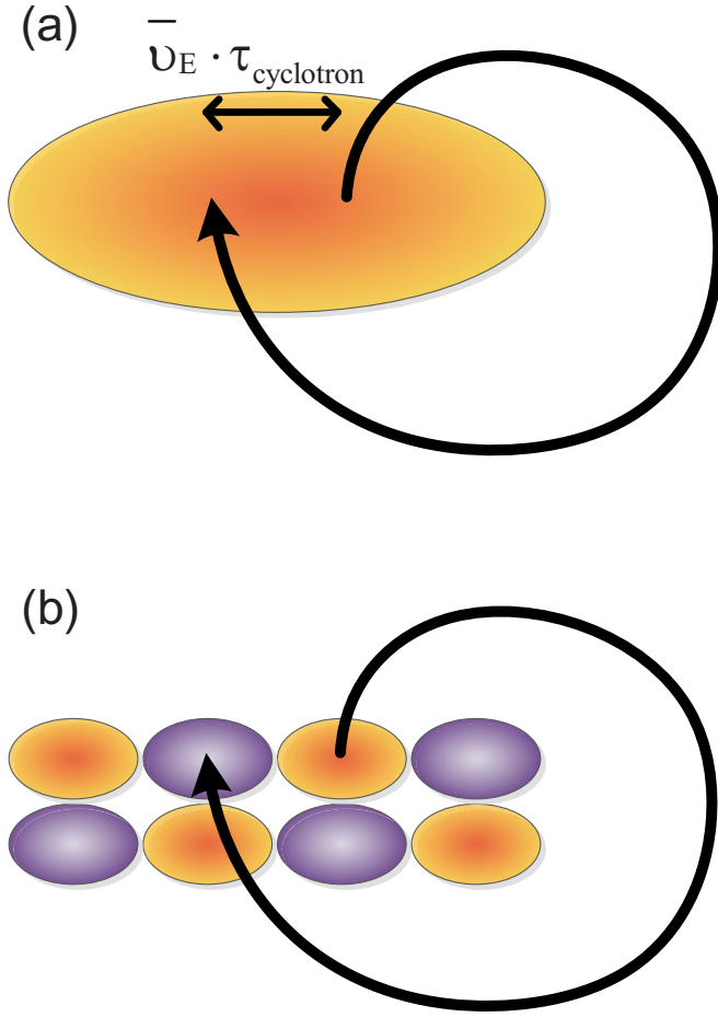
FIG. 12. (Color online) (a) The fast ion is correlated with the turbulent potential structure if the drift of gyrocenter during each cyclotron orbit is much smaller than the correlation length of the turbulence. (b) The fast ion is easily decorrelated with the wave if the drift is comparable with the correlation length of the turbulence, thus the fast ion orbit samples a different turbulent potential structure during each cyclotron orbit.
