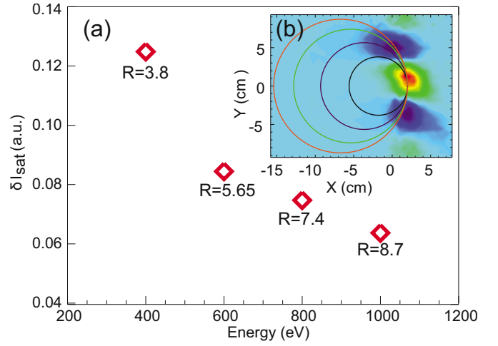
FIG. 11. (Color online) (a) The gyroaveraged density fluctuation shows a large reduction of fluctuation amplitude, and the fluctuation amplitude decreases with increased fast ion energy. (b) The cross-spectrum of the drift wave, measured by two triple probes two ports away (63.9 cm) from each other. The four measured gyroradii are overlaid.
