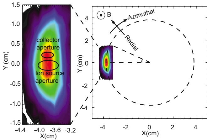
FIG. 5. (Color online) (right) Projection of the fast ion orbit onto the horizontal plane, with the beam profile measured three ports from the source overlaid. (left) Detail of the beam profile, together with the projection of the ion source and collector apertures.
