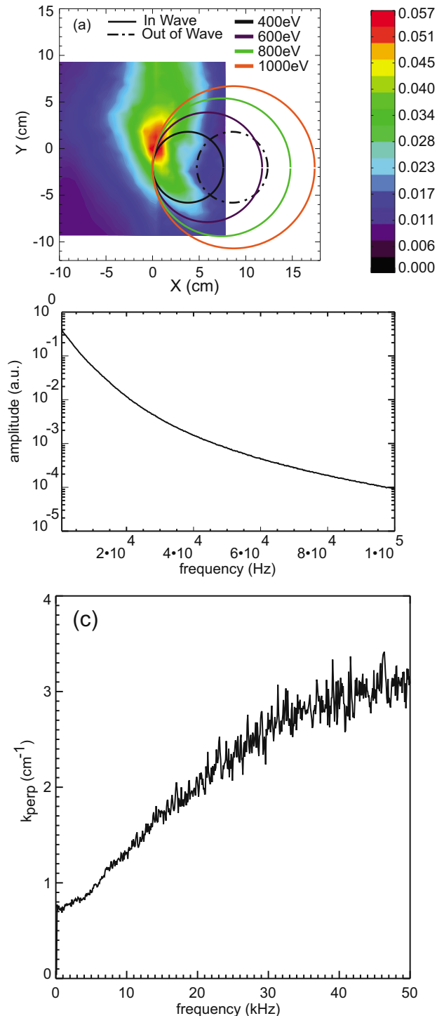
FIG. 4. (Color online) Characteristics of drift wave turbulence created by the plate-obstacle. (a) Contour of the total power of the wave with frequency ranges of 0.7–100 kHz, fast ion orbits with different energies is overlaid to show the overlap between the waves and particles. (b) Averaged fluctuation power spectrum (log-log). (c) Dispersion relation of the wave, calculated from the cross-correlation between two triple probes.
