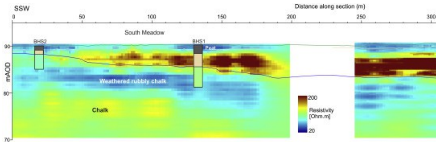
Fig. 12. Slice through interpolated 3D ERT model (see Fig. 14 for the location of the two separate blocks) showing the thinning of high-resistivity gravels (warm colours) towards the SSW. See Chambers et al. (2014) for additional information on the ERT survey and Fig. 5 for key to simplified borehole logs.
