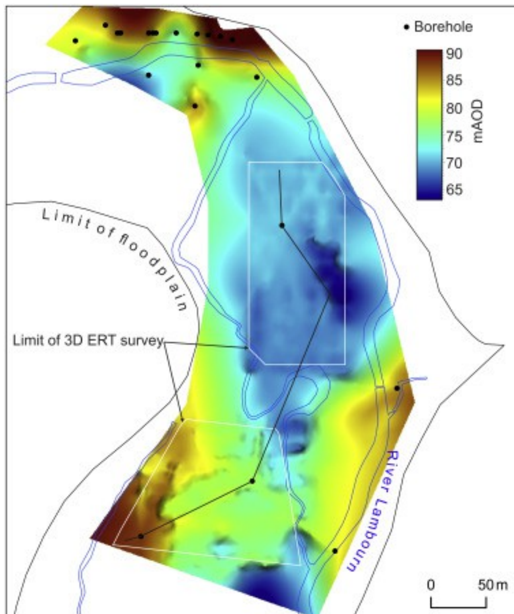
Fig. 11. Interpolated surface on the Chalk rockhead (base of the gravels) based on 3D ERT surveys and boreholes .
