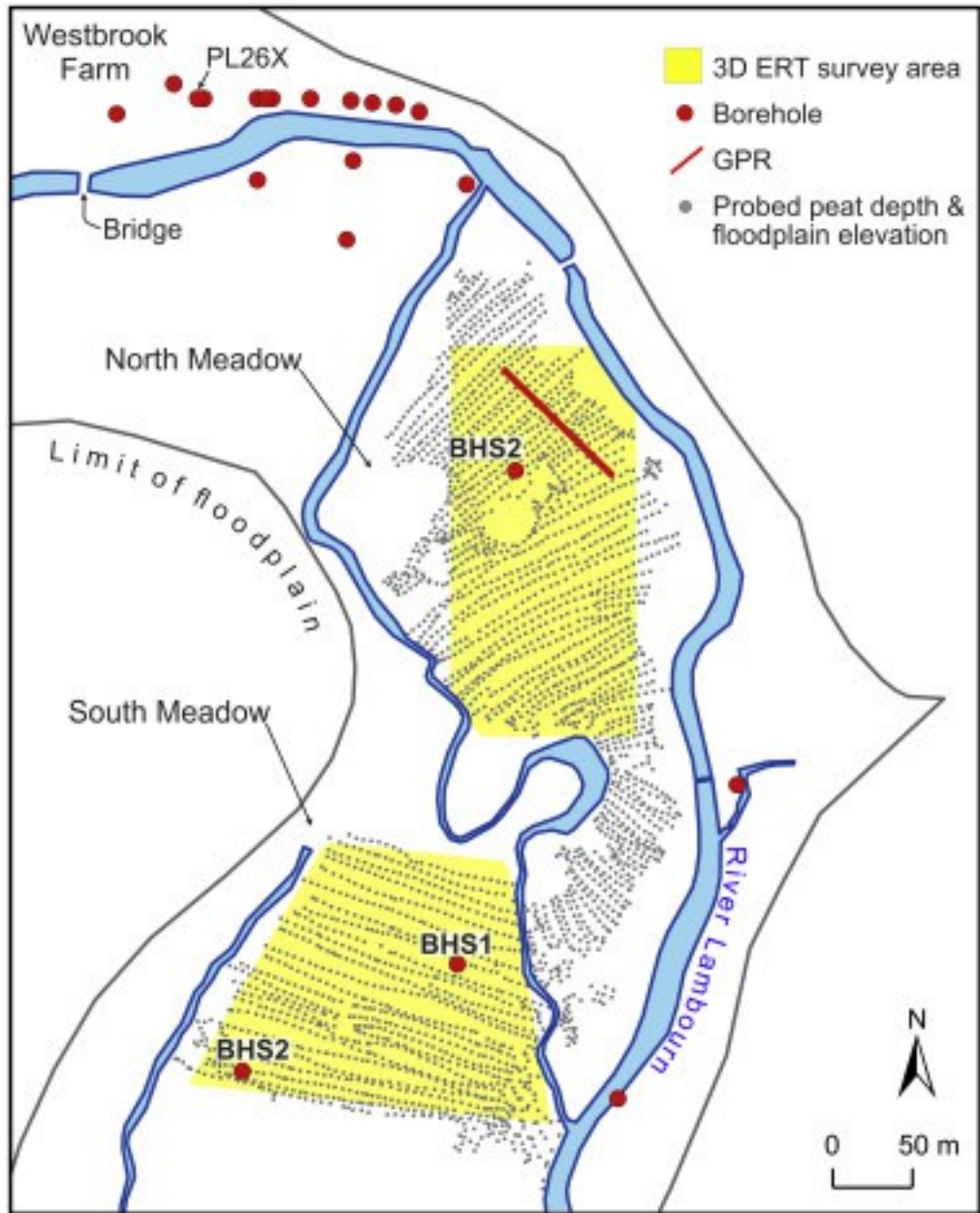
Fig. 6. Map showing the Boxford site and the distribution of boreholes , probed peat depths (and floodplain elevation points), 3D ERT survey areas and GPR line. Boreholes discussed in the text are labelled. Contains Ordnance Survey data ® Crown copyright and database right (2010).
