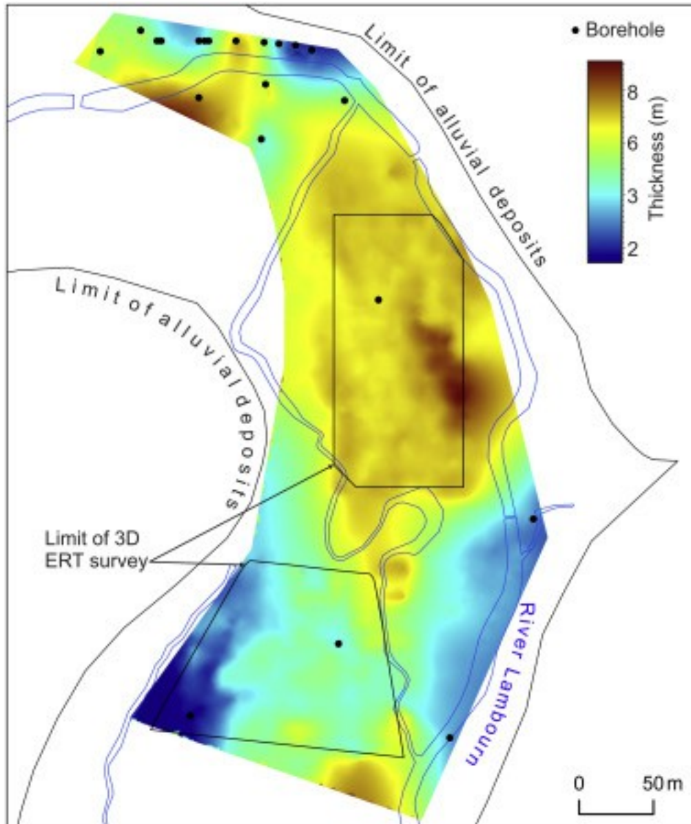
Fig. 8. Thickness map of Quaternary deposits overlying the Chalk based on the interpolation of data from 3D ERT ( Chambers et al., 2014 ) and boreholes .
