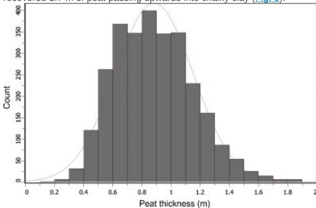
Fig. 16. Histogram showing distribution of peat thickness from 2815 probe measurements (see Fig. 7 for sample locations).
