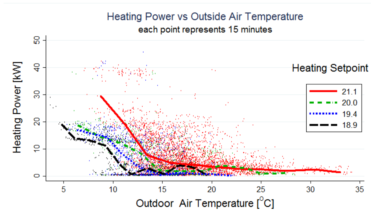
Figure 15– Heating power versus outdoor temperature
