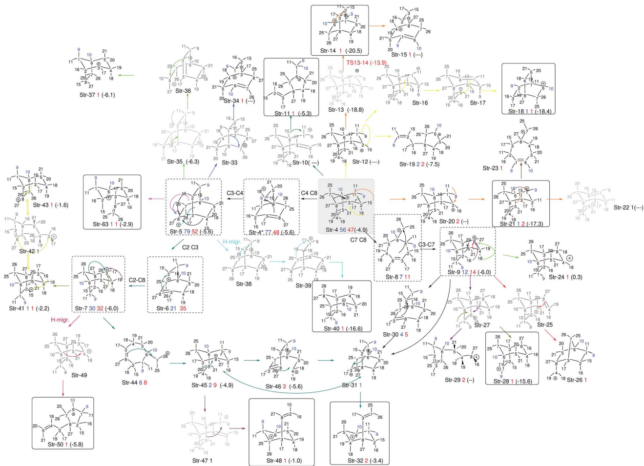
Fig. 8 Reaction paths followed by trajectories, depicted as sequences of structures with a defined connectivity. Structures in black correspond to those that appear in Fig. 7 (we use the prefix Str on their names to avoid confusion with other numbers used in the representation). Below each of those, a number in blue indicates how many times this structure appears at exactly the 1000 fs time step of a trajectory, and a number in red how many times it does so at 2000 fs. With dashed squares, we have highlighted those structures most frequently encountered, while we have used solid squares to indicate tertiary carbocations (perhaps surprisingly, they are not among those structures most frequently encountered at either 1000 or 2000 fs). All black structures in the scheme were used as starting points of geometry optimizations. For those where the optimization preserved connectivity (they are actual minima on the potential energy surface), their energies relative to 1-H are noted between parentheses. The numbers in blue on the structures represent the methyl groups that keep their structural integrity along the trajectory.
