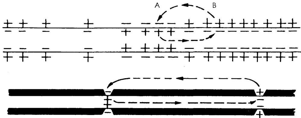
Diagrams illustrating the local circuit theory; the upper sketch represents an unmyelinated nerve fibre, the lower a myelinated nerve fibre.
