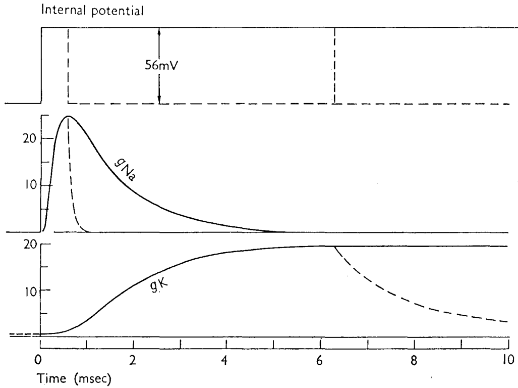
Time course of sodium conductance ( g_{Na} ) and potassium conductance ( g_K ) associated with depolarization of 56m V; vertical scale in mmho/cm 2 . The continuous curves, which were derived from those in Figure 27, are for a maintained depolarization; broken curves give the effect of repolarizing the membrane after 0.6 or 6.3 msec. (From Hodgkin, 1958, based on Hodgkin & Huxley, 1952a & b.)
