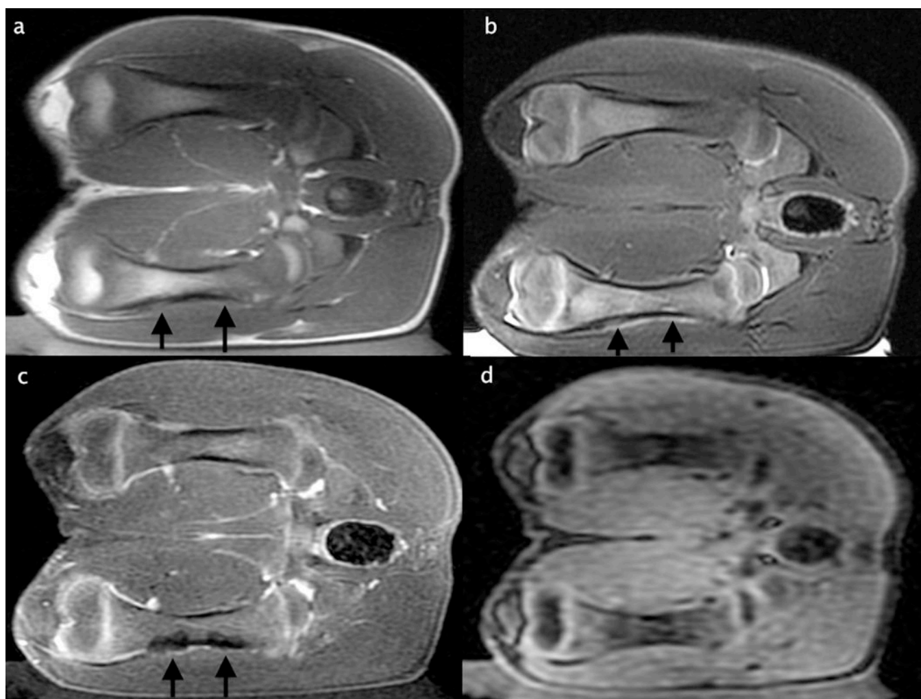
Figure 2. Coronal (a) T2-weighted, (b) T1-weighted, (c) contrast enhanced T1 spoiled gradient echo and (d) perfusion MR images. The proximal and distal diaphysis of the right femur (downside limb) was sonicated. MR images were acquired immediately following HIFU ablation. The ablations are best seen on contrast enhanced T1 spoiled gradient echo imaging with two focal ovoid regions of hypoenhancement (arrows). Subtle T2 hyperintensity is noted along the diaphysis (arrows). Perfusion imaging failed to demonstrate the ablations.
