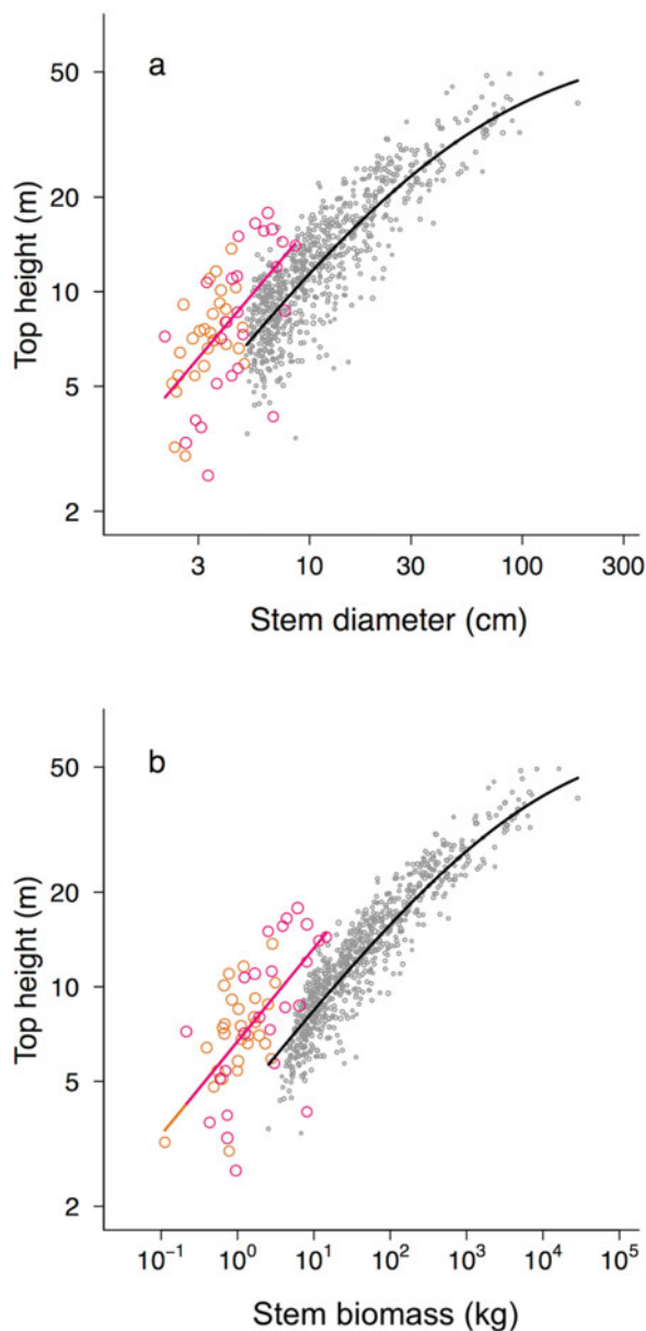
Figure 2. Allometric properties of bamboo ramets and woody trees in a Malaysian hill rain forest. Ramet (stem) top height ( H_{\text{ramet}} , H_{\text{tree}} ) on culm (stem) diameter at breast height ( D_{\text{culm}} , D_{\text{tree}} ) (a) and on culm (stem) biomass ( W_{\text{culm}} , W_{\text{stem}} ) (b) for Gigantochloa ligulata (orange), Schizostachyum grande (pink) and woody trees (grey). Solid lines show the allometric predictions.
