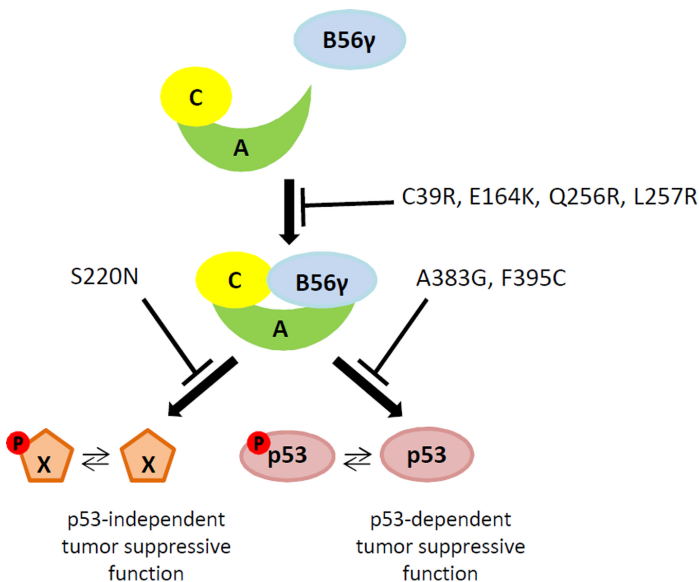
Figure 5. Inactivation of B56γ-PP2A tumor-suppressive function by B56γ mutations
