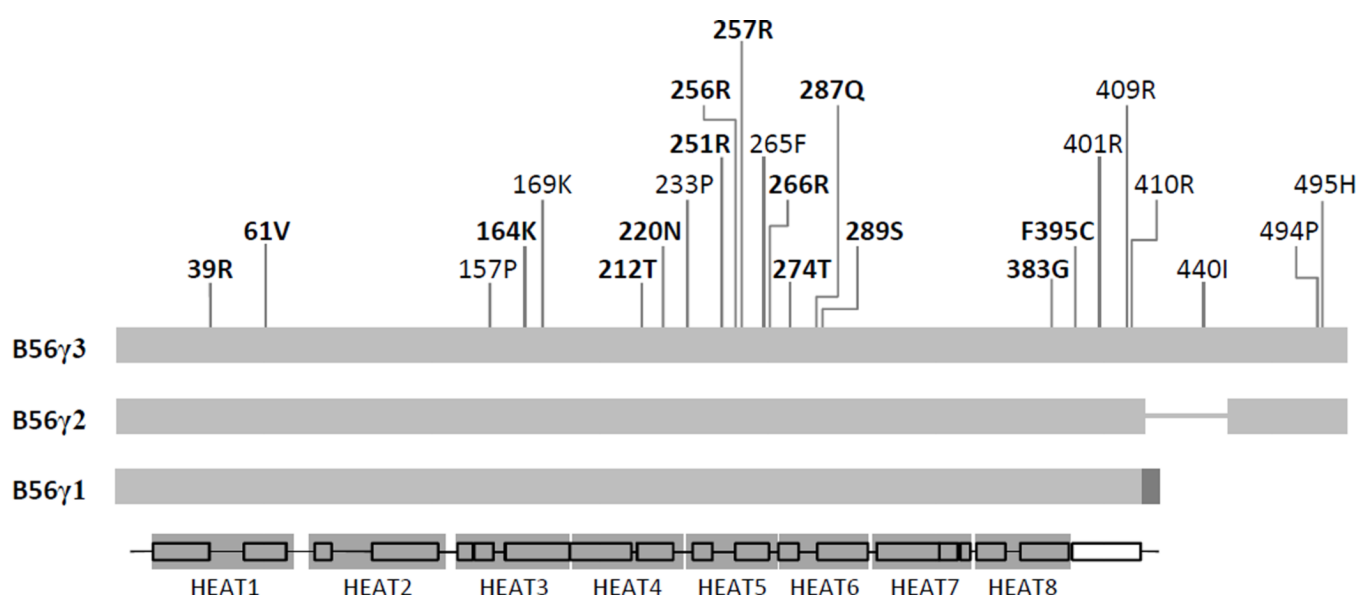
Figure 1. Distribution of B56γ mutations identified by AceView
