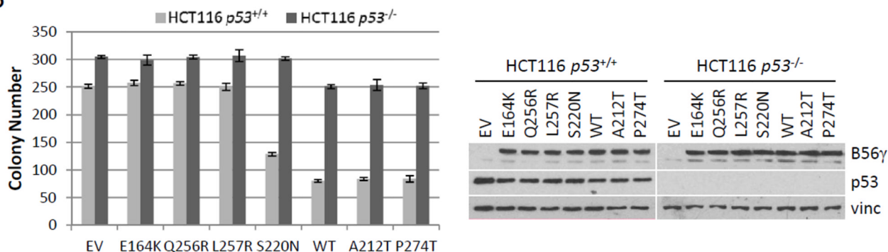
Figure 2. Effect of B56γ mutants on tumor suppressor function
