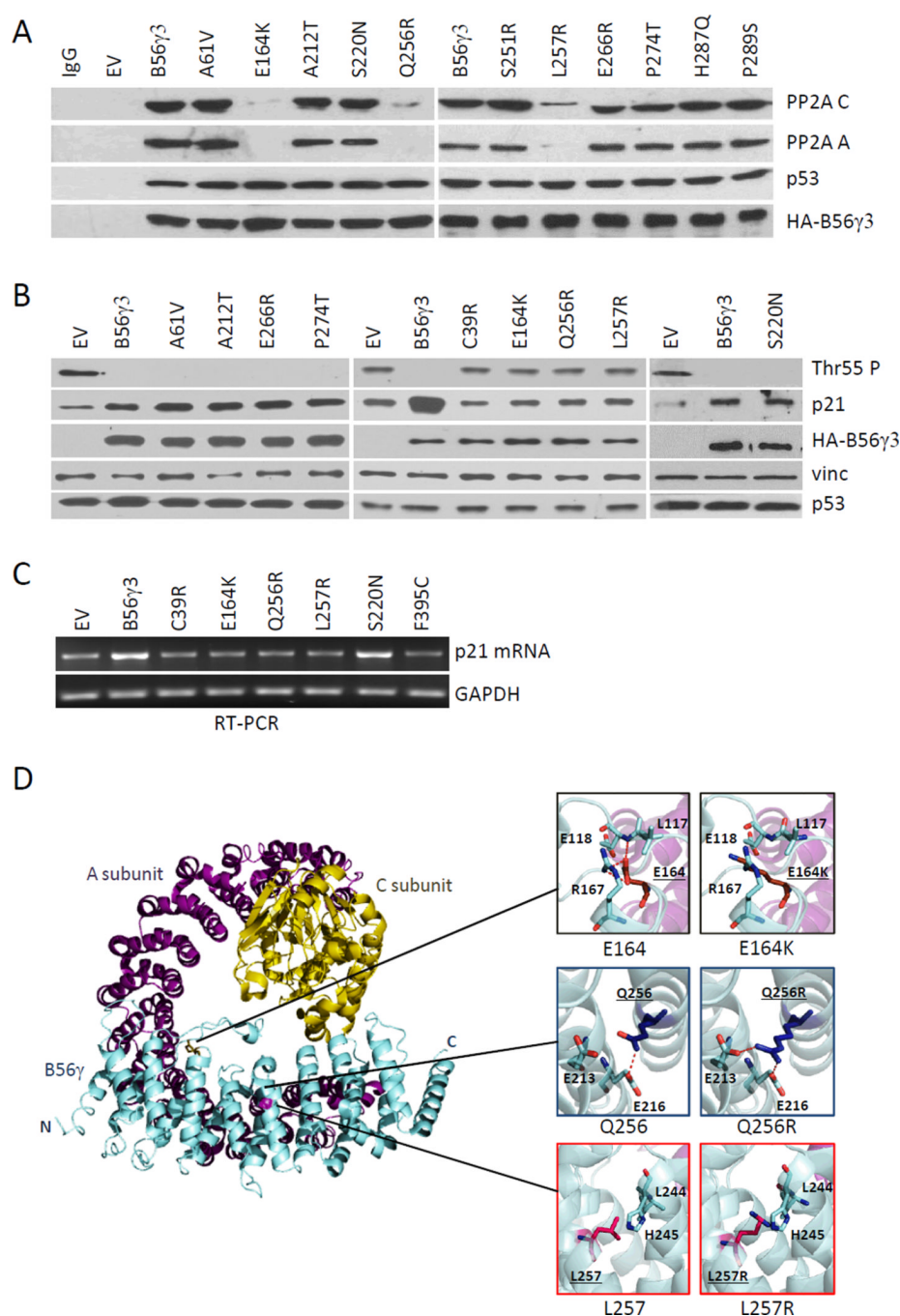
Figure 3. Interaction of B56γ mutants with PP2A A and C and p53
