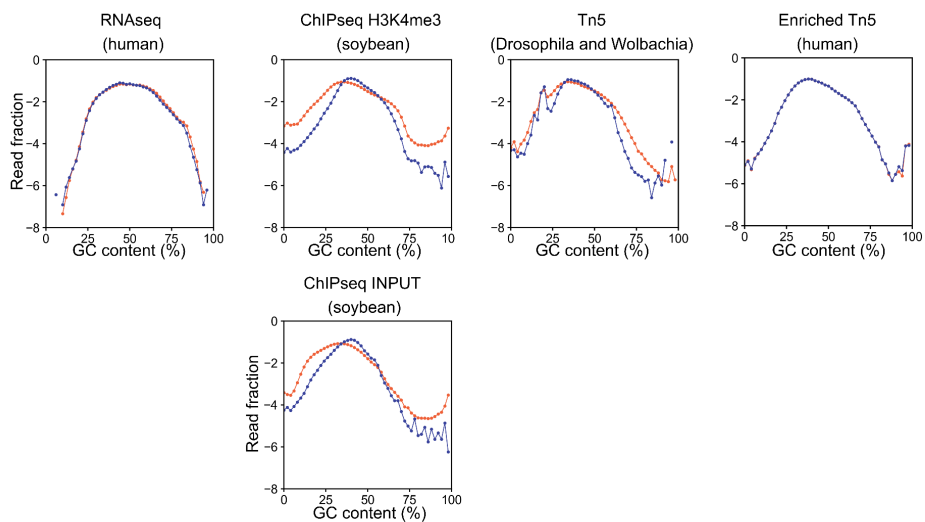
Fig. S2: GC-content of Illumina and R2C2 reads sampling from the same library. \text{Log}_{10} converted read fractions of reads with different GC content is shown for all experiments performed for this study. For the ChIPseq study, read fractions for both libraries in the analyzed pool are shown (H3K4me3 and INPUT). Illumina reads are shown in orange and R2C2 reads are shown in blue.
