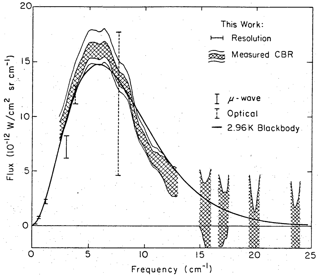
Figure 1. Second Berkeley spectrum plotted as \pm 1 \sigma error limits with a distinction made between two types of experimental error. The cross-hatched region gives the error limits considering only those sources of error which are essentially statistically independent between one spectral resolution element and the next. When sources of error are included which affect the overall scale factor the crosshatched region can be shifted up or down within the limits indicated by the thin solid lines. For comparison we also show the spectrum of the 2.96 K blackbody which fits the measured integrated flux, as well as selected microwave and optical measurements of the cosmic background radiation.
