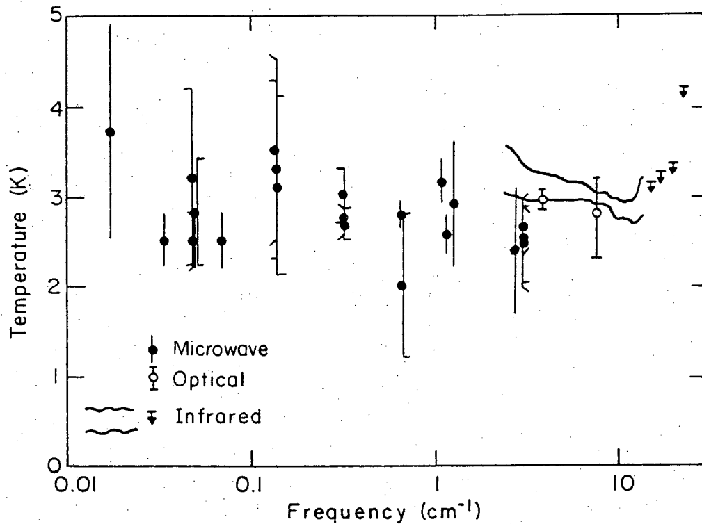
Figure 2. Collected microwave, interstellar CN and Berkeley results plotted as a frequency dependent thermodynamic temperature. The error limits are intended to be \pm 1 \sigma .
