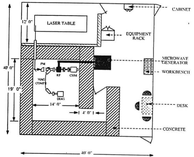
Fig. 5 Sample BES Layout
