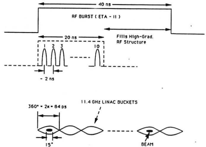
Fig. 1 Required Pulse Train Characteristics for 1-GeV Text Expt.
