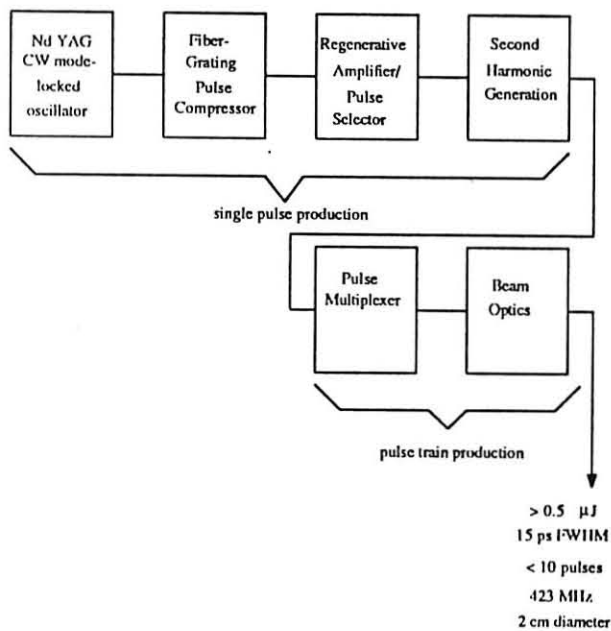
Fig. 4 Block Diagram of Laser Source
