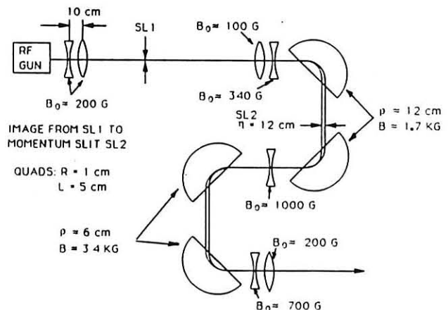
Fig. 3 BES Magnetic Bunch Compressor
