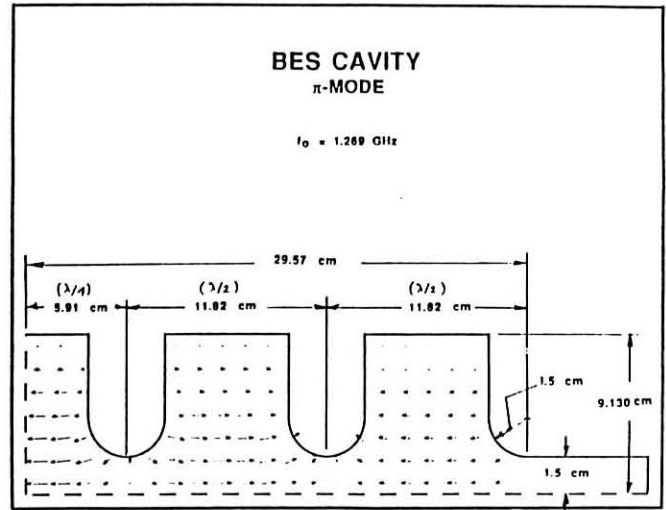
Fig. 2 Electric field distribution in BES cavity.
