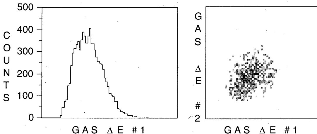
FIG. 3-8: Gas- \Delta E Signals. On the left, gas- \Delta E signals are shown for the 386 keV beta-delayed proton group of ^{25}\text{Si} . On the right, a \Delta E_2 vs. \Delta E_1 correlation plot is shown for the same 386 keV proton events from the peak in the spectrum on the left.
