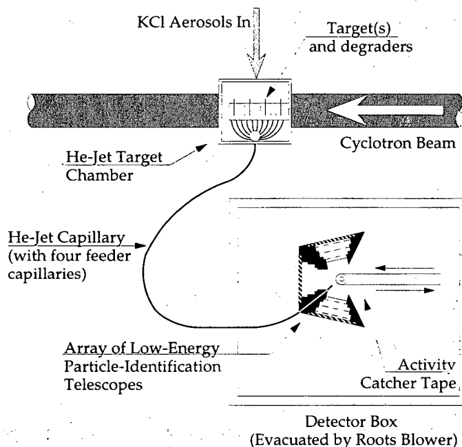
FIG. 4-5: Experimental set-up for the first low-energy measurements. Note that the size of the detector array is somewhat exaggerated.
