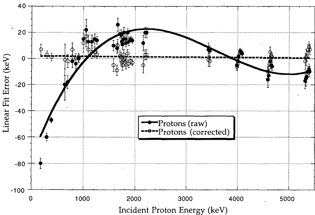
FIG. 3- 16: Proton calibration fit data. The x-axis shows the energies of the calibration points, either taken directly from the literature (undegraded proton peaks) or from the literature values minus the calculated energy losses in the Al degrader foils. The y-axis shows the deviation of the calculated energies of individual peaks (based on the calibration) from the correct values [Fit Error = E(\text{from calibration}) - E(\text{correct}) ].
