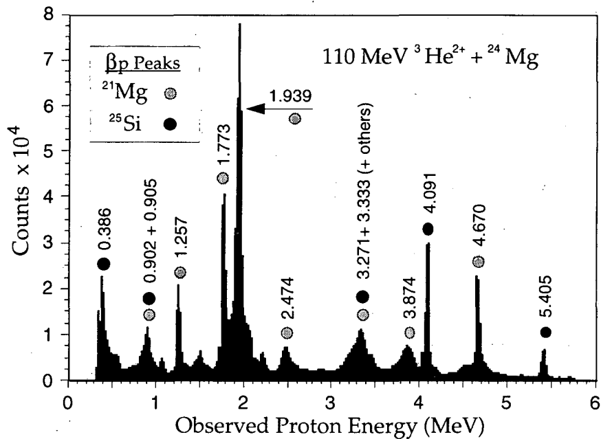
FIG. 5- 3: Beta-delayed proton spectrum, E < \sim 6 MeV. These protons were stopped in the first Si detector. Peaks from ^{25}\text{Si} and ^{21}\text{Mg} beta-delayed proton decays, used for calibration, are indicated.
