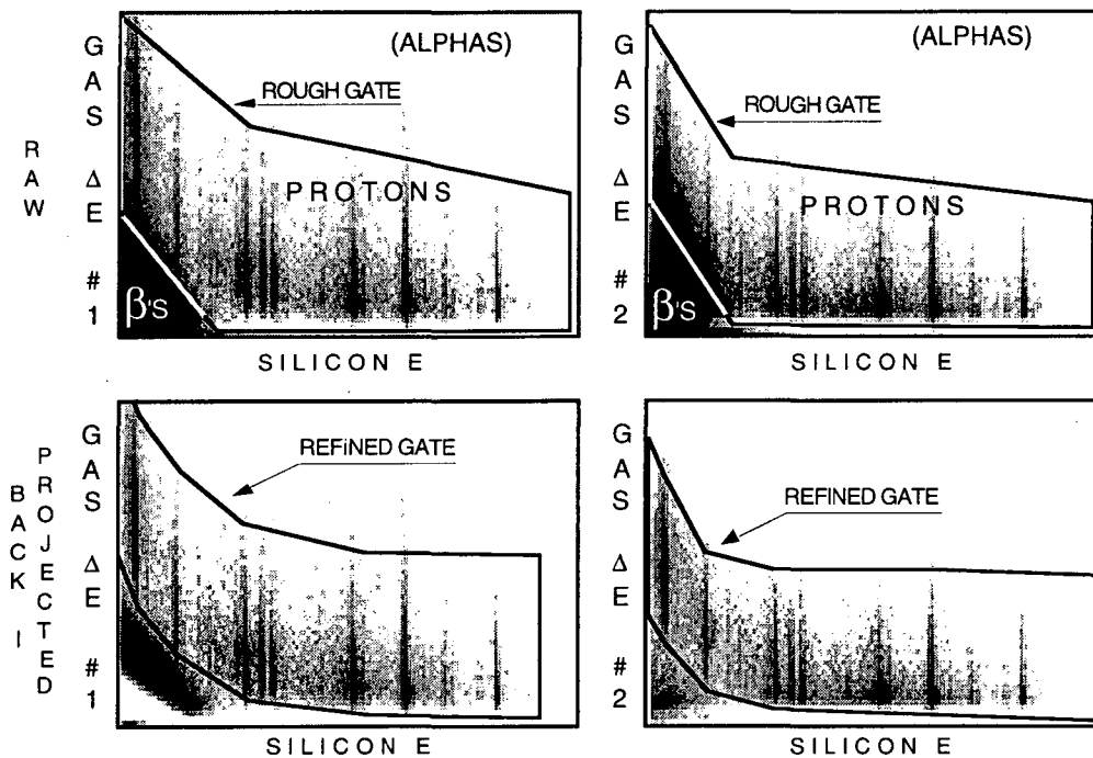
FIG. 3-12: Standard back-projection gating. The upper two-dimensional spectra show the data prior to gating. The two lower spectra contain the subsets of the data in the upper spectra which fell within the "rough" gates defined in the upper spectra. See text.
