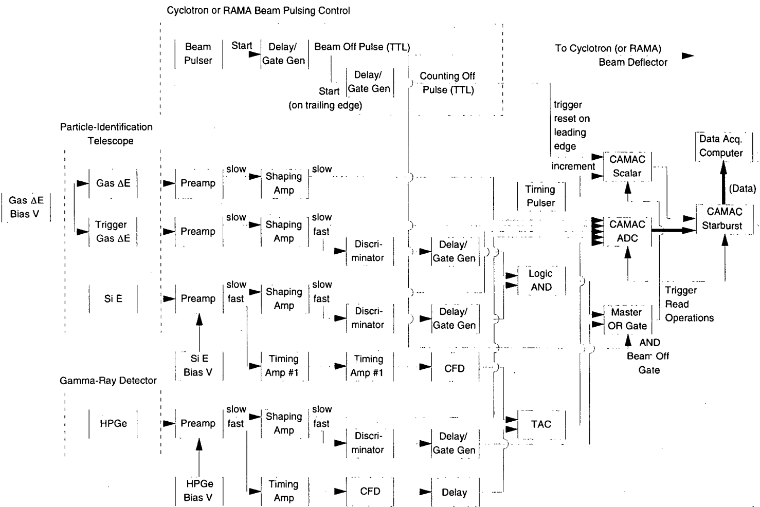
FIG. 3-11: Generalized counting electronics. See text for an explanation of abbreviations and functions of individual modules.
