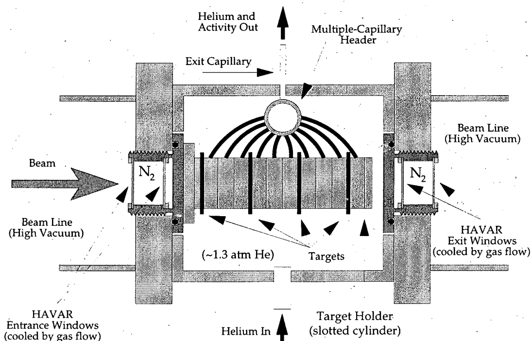
FIG. 3-3: Helium-jet target. In the multiple-capillary system shown, ten small capillaries sweep the activity from behind each of ten target-holder slots. These small capillaries then feed into the single exit capillary. In the configuration shown, a target is placed in every third slot; the other slots are left empty.
