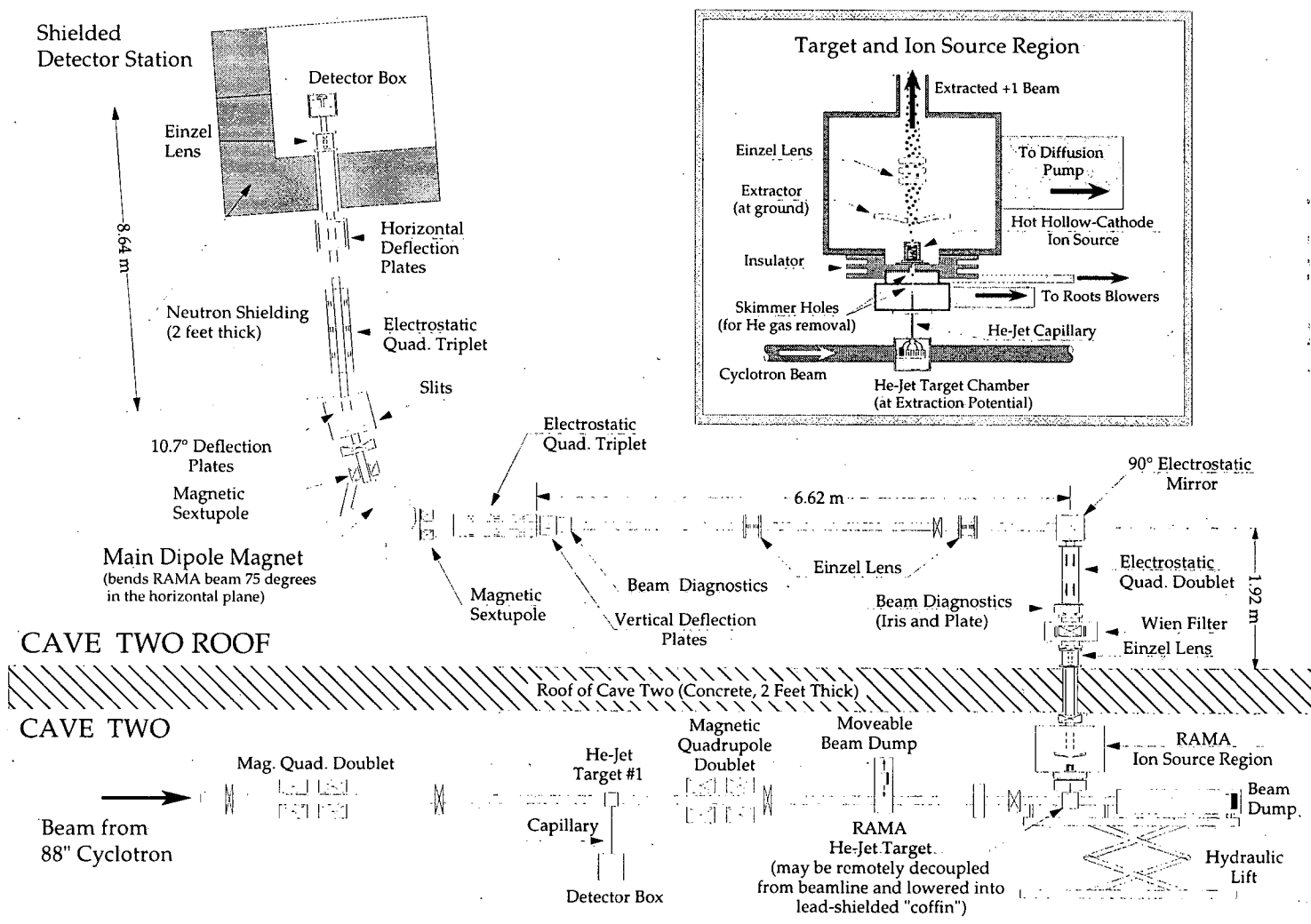
FIG. 3-4: Schematic diagram of the Cave 2 beam line and RAMA. The inset at upper right shows the He-jet target, skimmers and ion-source/extractor box.
