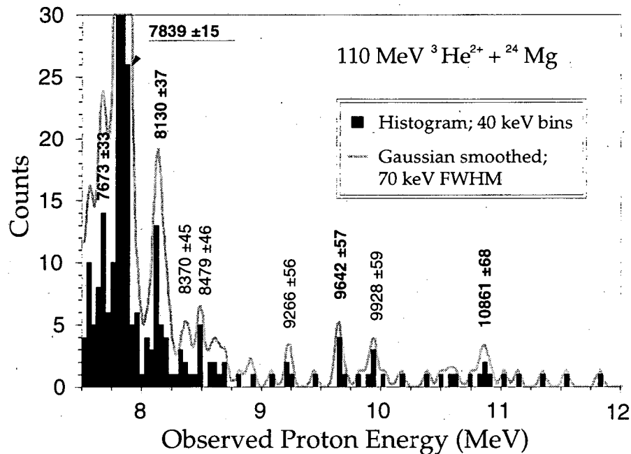
FIG. 5- 5: Proton spectrum, 7.5 \text{ MeV} < E < 12.0 \text{ MeV} . The gray line indicates the results of a Gaussian smoothing operation applied to the data. The known beta-delayed proton peaks of ^{22}\text{Al} are indicated, as well as other potential new peaks.
