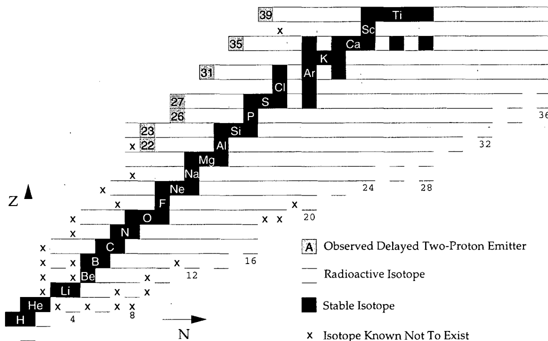
FIG. 2- 6: Region of the Chart of Nuclides where beta-delayed two-proton decay has been observed.
