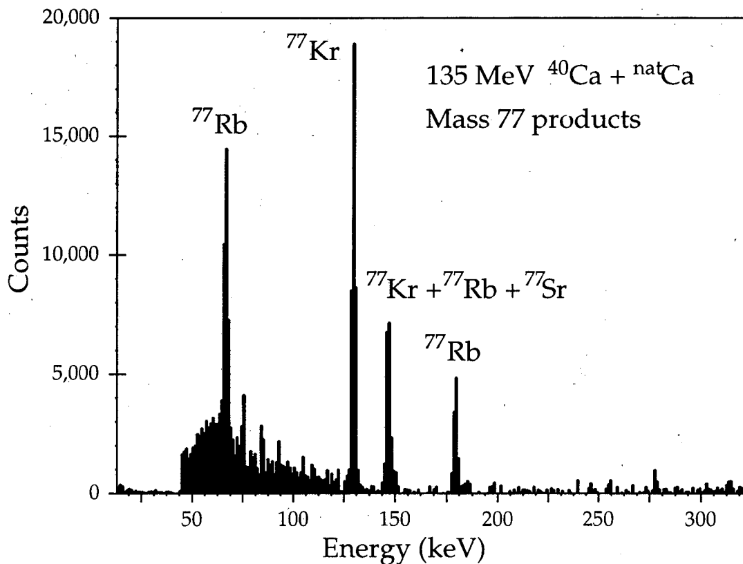
FIG. 6-3: Gamma-ray spectrum of mass-77 reaction products. The spectrum of long-lived species, taken during the 24 hour period after the main experiment was completed, has been subtracted.
