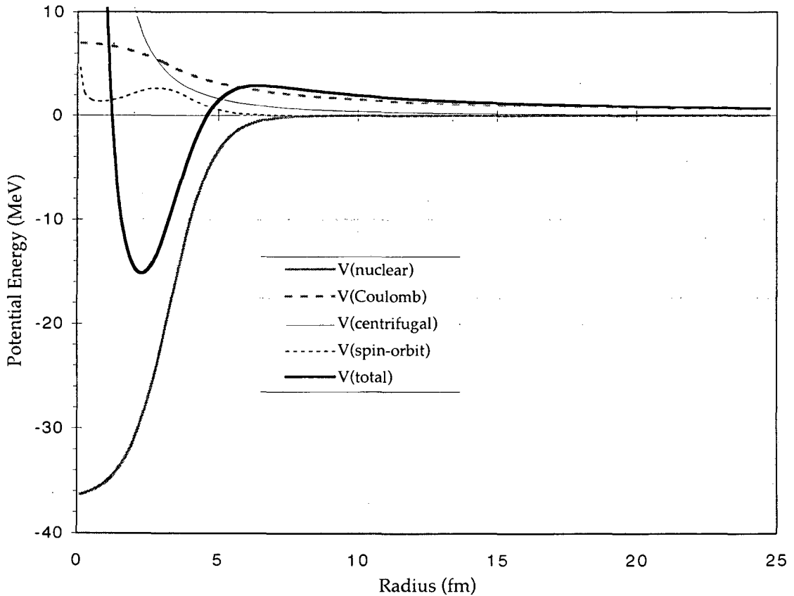
FIG. 2-2: Potential barrier for proton decay from the IAS of ^{23}\text{Al} , calculated from the optical-model parameterization of Becchetti and Greenlees (Bec69) for an l=0 decay from the 0d_{5/2} orbital.
