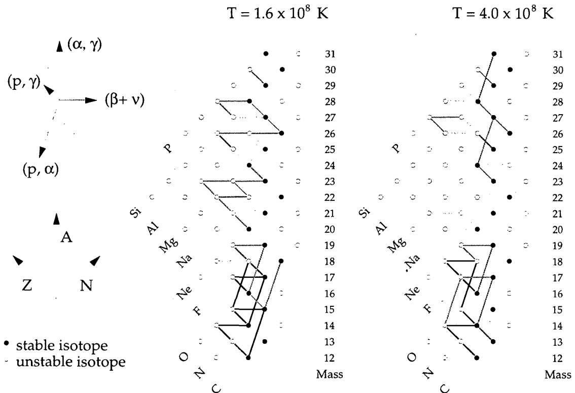
FIG. 2- 10: Reaction pathways in explosive hydrogen burning processes in novae at two temperatures, as calculated by Wiescher, et al. (Wie86a). The darkness of the lines is an indication of the flux strength.
