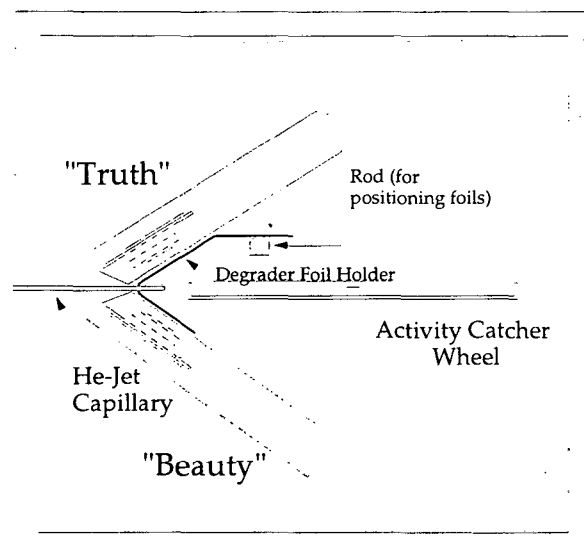
FIG. 4- 10: Detector configuration for the second low-energy measurements of the decay of ^{23}\text{Al} .
