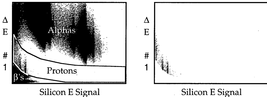
FIG. 4-6: \Delta E vs. E spectra, 40 MeV p + ^{nat}\text{Mg} bombardment. On the left, the raw data are shown prior to gating; the alpha, beta and proton regions are indicated. On the right, the proton events are shown after data reduction.
