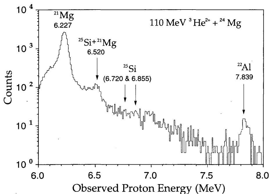
FIG. 5- 4: Proton spectrum, 6 \text{ MeV} < E < 8 \text{ MeV} . The peaks at 6.227 and 7.839 MeV were used for calibration. The expected energies of other weak proton groups are also indicated.
