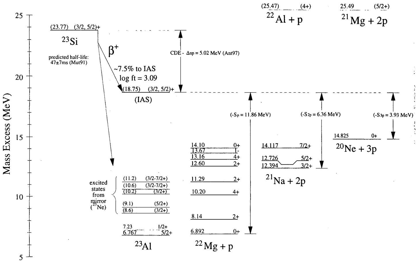
FIG. 5-2: Predicted decay scheme for ^{23}\text{Si} . The mass excess of ^{23}\text{Si} is taken from Aud95; the energy of its isobaric analog state is derived from a Coulomb displacement energy calculation.
