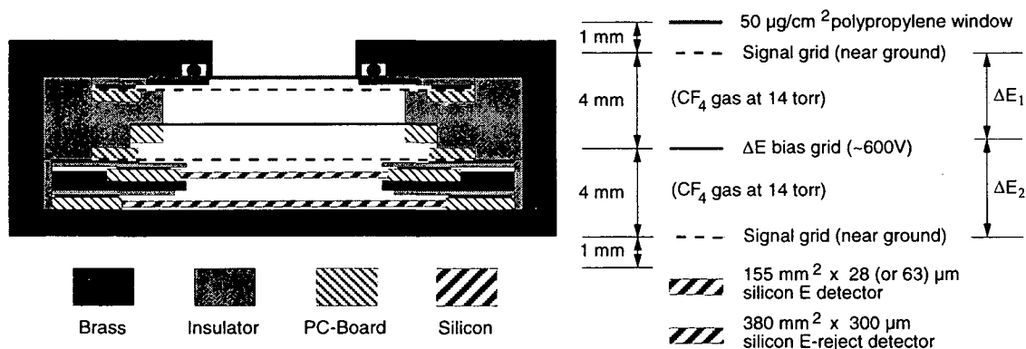
FIG. 4-9: Cross-sectional view of a modified low-energy particle-identification telescope with improved beta-particle rejection, used in the second series of measurements of the decay of ^{23}\text{Al} .
