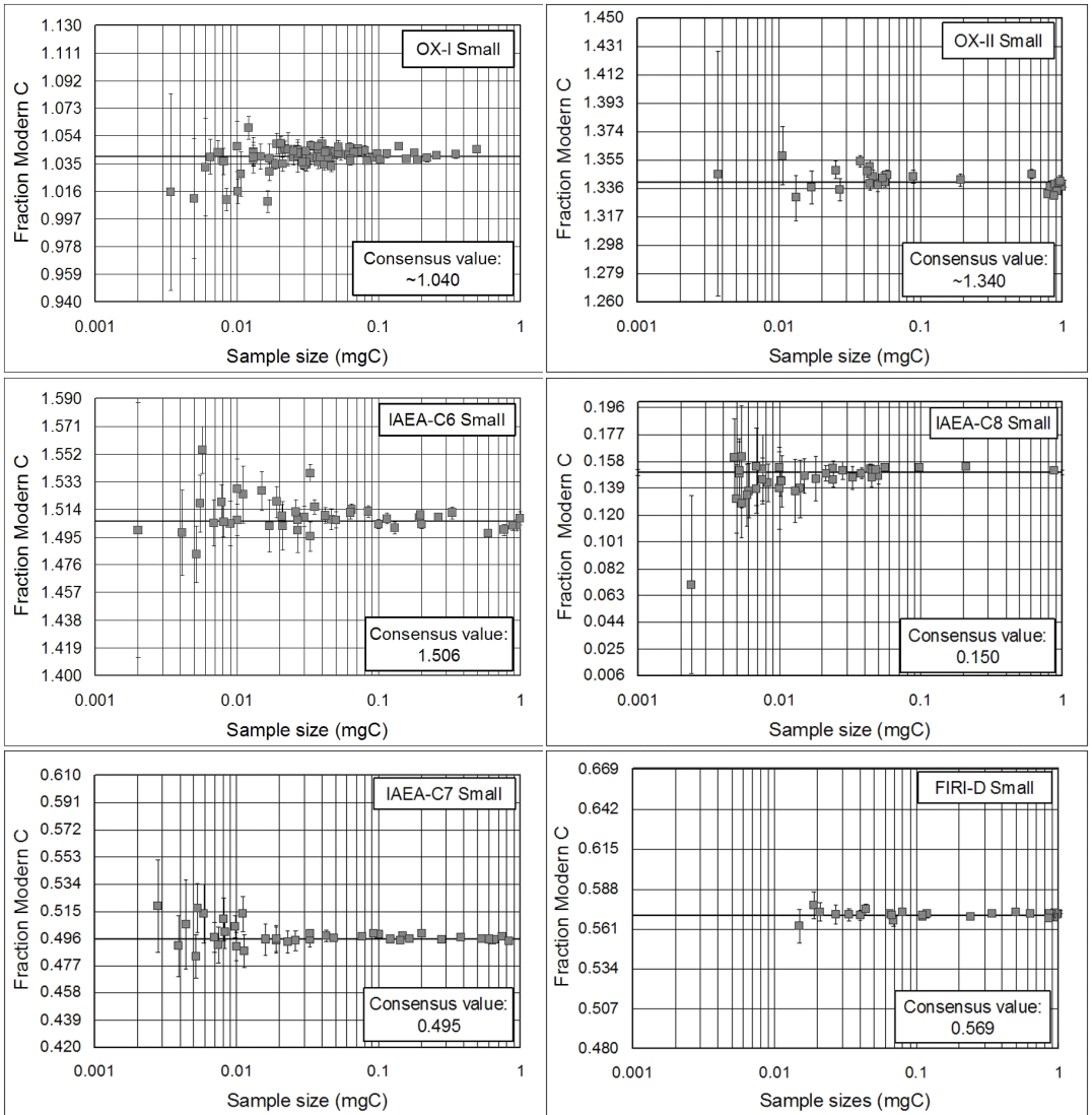
Figure 8 Fraction modern C results for the OX-I, OX-II, IAEA-C6, -C7, -C8, and FIRI-D samples between 0.002 and ~1 mg C from multiple AMS ^{14}\text{C} measurements performed between July 2005 to May 2006 on small and ultra-small sample wheels. Results were normalized and blank corrections applied as for Figure 7.
