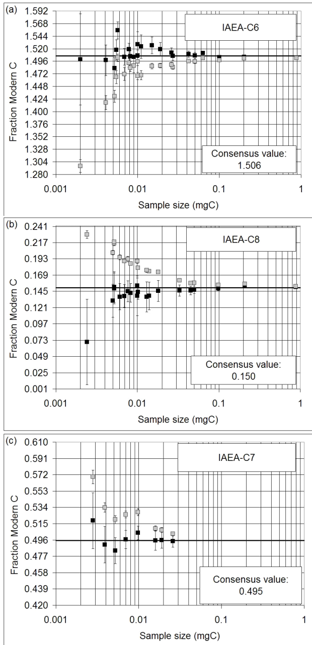
Figure 7 Fraction modern C background-corrected values (black) and uncorrected values (gray) for IAEA-C6, -C7, and -C8 samples between 0.002 and \sim 1 mg C from 2 wheels of small and ultra-small samples, illustrating the effects of modern and dead contamination on secondary standards. These results were normalized to sets of 6 OX-I standards. For samples in the tens of micrograms range, this set was composed of regular graphite targets (1 mg C). For ultra-small samples ( <0.010 mg C), the normalizing standards were \sim 0.010 mg C. Mass-balance blank corrections have been applied using the formulae presented in Santos et al. (2007b: Section 2.8 and Appendix A), with uncertainties derived from the scatter in the blank data. When blank corrections are not applied (and errors are only statistical), a mass dependence due to a constant contamination is observed. When small secondary standard values are near-modern, the dead contamination is dominant (a); when they are close to background values, the modern contamination is dominant (b); and when values are close to half-modern, they are equally sensitive to both contaminations, but the larger modern blank has more effect (c).
