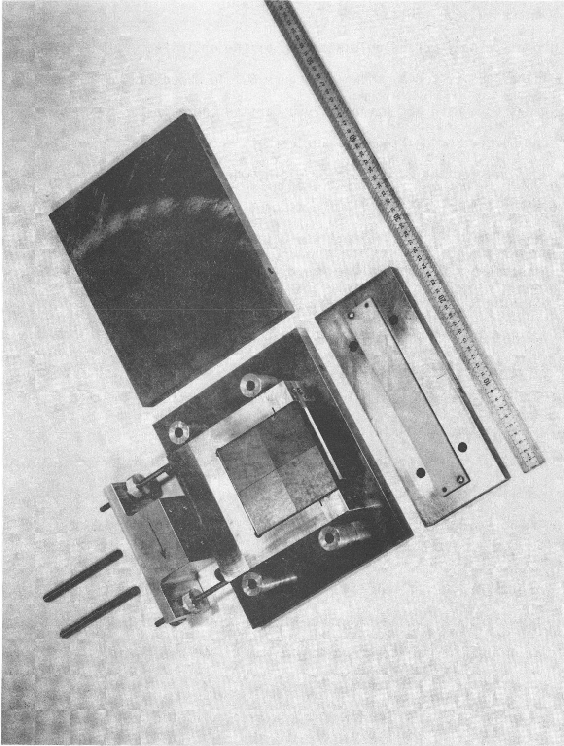
Wiggler Prototype Half Period Test Assembly Figure 8
