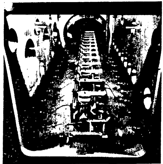
Fig. 3: View (towards gun) of transport and matching quadrupoles.
