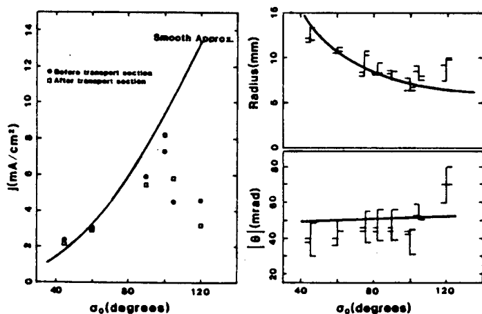
Fig. 4: Measured current density, beam radius, and envelope divergence (curves are calculated matched values).
