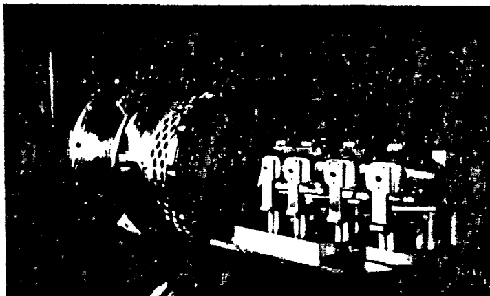
Fig. 2: The gun with four matching quadrupoles in place.
