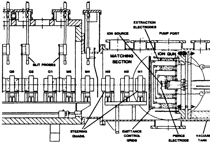
Fig. 1: A drawing of the gun showing emitter with Pierce electrode, separately controlled electrodes, and emittance control grid.
