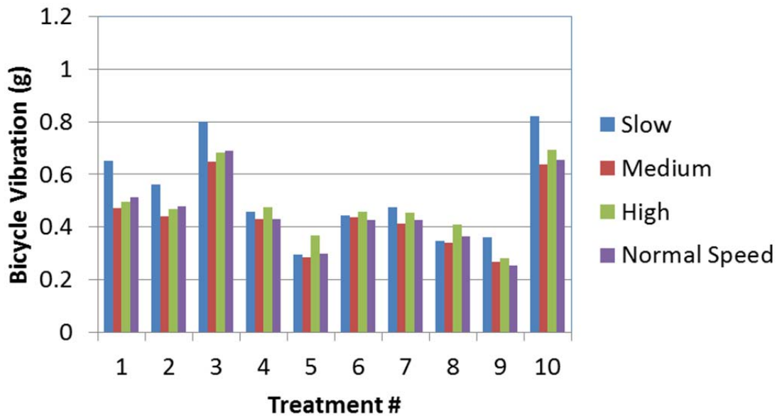
Figure 4.18: Bicycle vibration measured at different speeds on the Mon-198 test sections. (See Table 3.4 for a description of each treatment #; Normal Speed indicates different speeds for different riders.)
