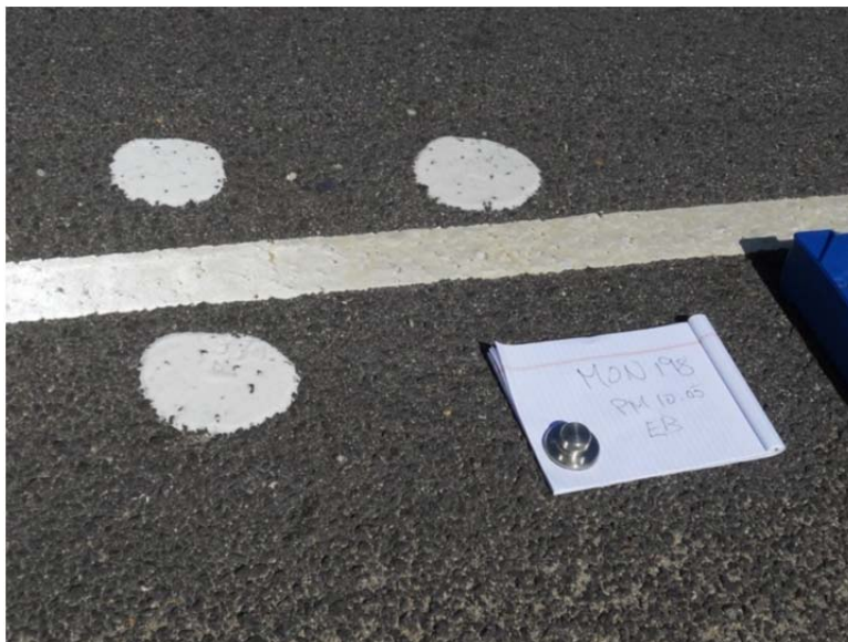
(b) Mon-198 PM 10.05 coarser 3/8" gradation chip seal
