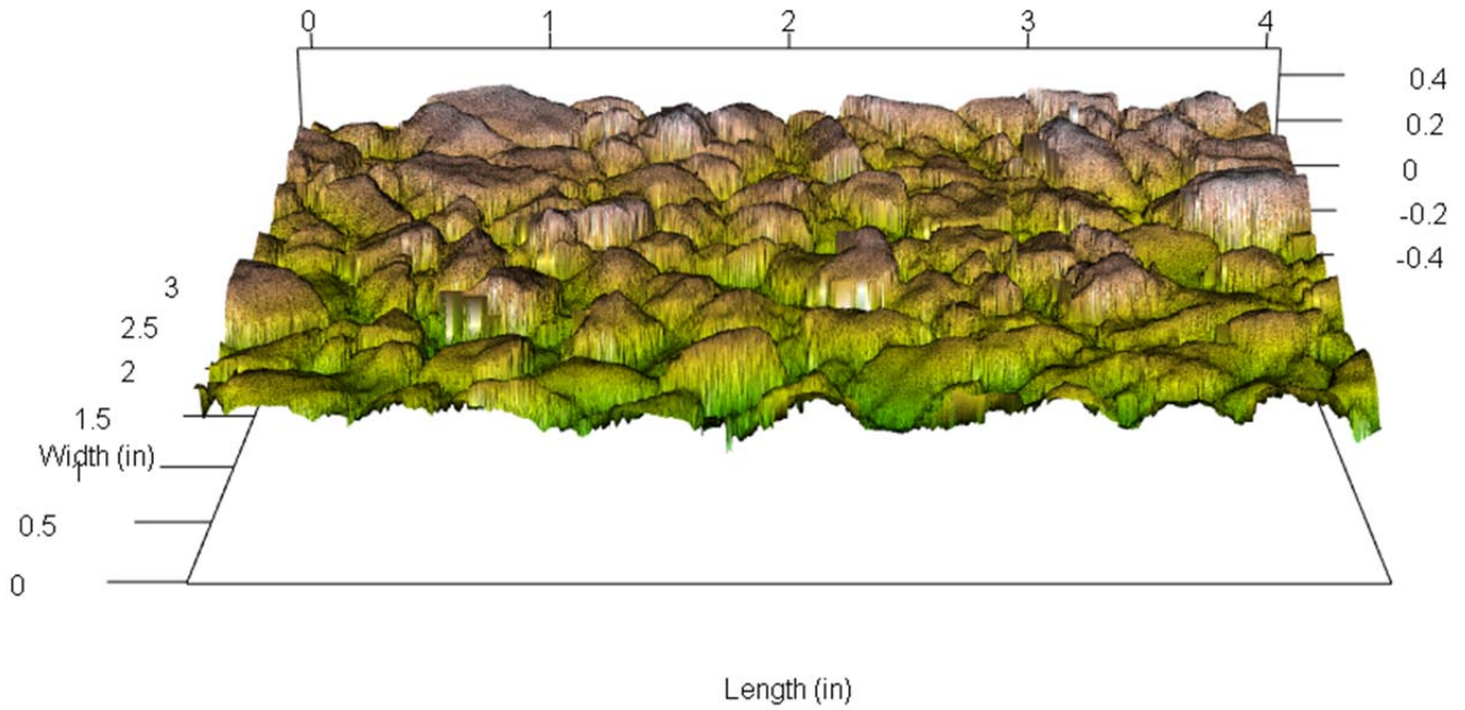
#3 Modified Binder Seal Coat - Utilizing a Steel Roller (PM 4.9-5.1)
