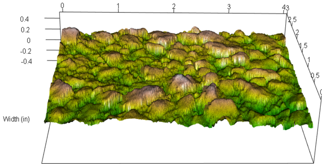
Length (in) (c) Dense-graded asphalt overlay on Mon-198 EB PM 6.81
