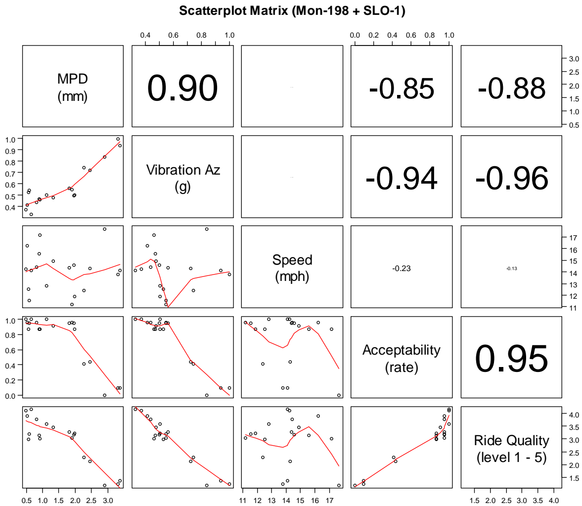
Figure 4.24: Correlations between MPD, acceleration, bicycling speed, acceptability, and ride quality level (Mon-198 test sections).
