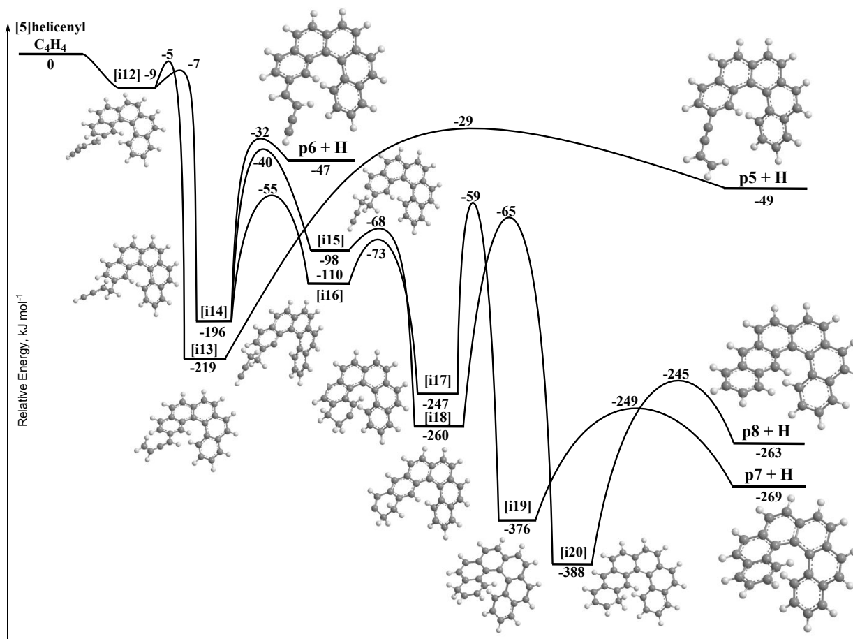
Fig. 5. Potential energy surface (PES) for the [5]helicenyl ( \text{C}_{22}\text{H}_{13}\cdot ) reaction with vinylacetylene ( \text{C}_4\text{H}_4 ) leading to [6]helicene ( \text{C}_{26}\text{H}_{16} ). This PES was calculated at the G3(MP2,CC)//B3LYP/6-311G(d,p) level of theory. The relative energies are given in \text{kJ mol}^{-1} .
