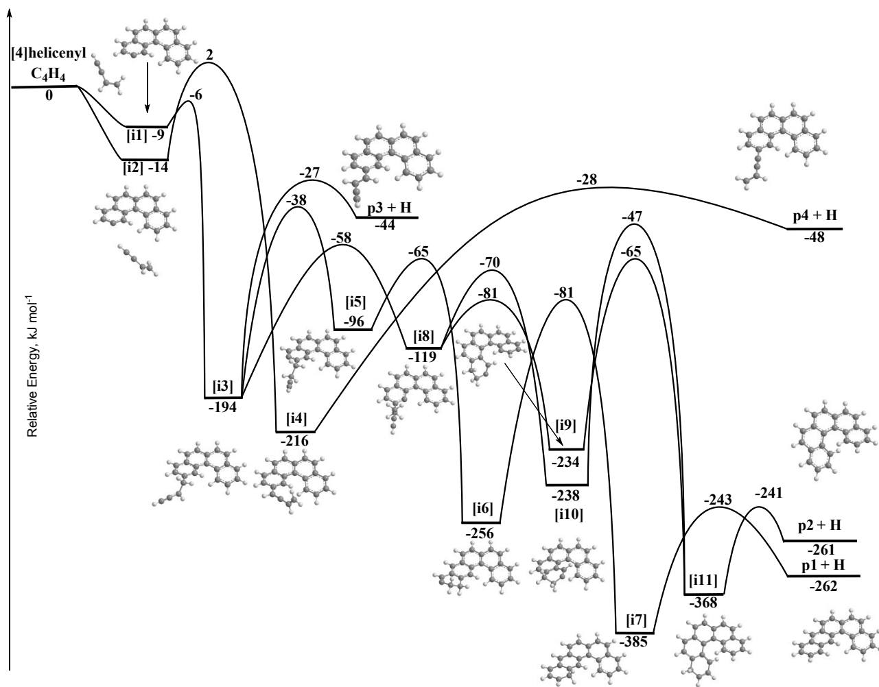
Fig. 4. Potential energy surface (PES) for the [4]helicenyl ( \text{C}_{18}\text{H}_{11}\bullet ) reaction with vinylacetylene ( \text{C}_4\text{H}_4 ) leading to [5]helicene ( \text{C}_{22}\text{H}_{14} ). This PES was calculated at the G3(MP2,CC)//B3LYP/6-311G(d,p) level of theory. The relative energies are given in \text{kJ mol}^{-1} .
