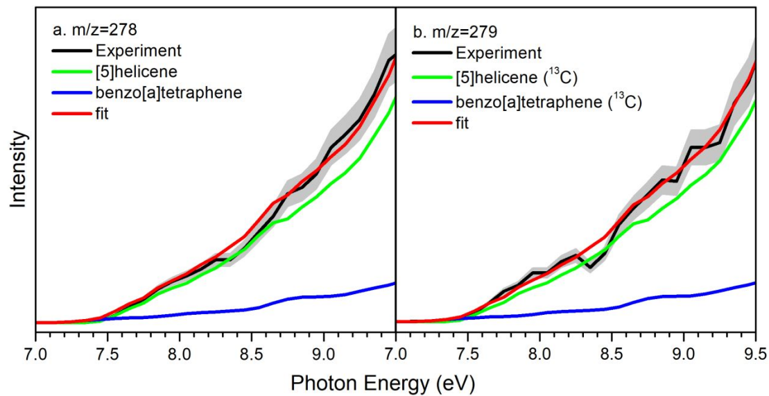
Fig. 3. Photoionization efficiency (PIE) curves of m/z = 278 and 279 for the reaction of 2-bromobenzo[ c ]phenanthrene ( \text{C}_{18}\text{H}_{11}\text{Br} ) - vinylacetylene ( \text{C}_4\text{H}_4 ). Black: experimentally derived PIE curves; colored lines (green and blue): reference PIE curves; red lines: overall fit. The overall error bars consist of two parts: \pm 10\% based on the accuracy of the photodiode and a 1\sigma error of the PIE curve averaged over the individual scans.
