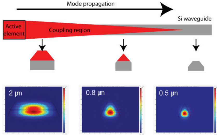
Figure 8.1: On the top: schematics of the III-V/Si beveled adiabatic taper coupler with cross-sections showing decreasing coupler widths. On the bottom: finite element simulations (COMSOL) of a fundamental TE-like mode for beveled waveguides with different widths.
