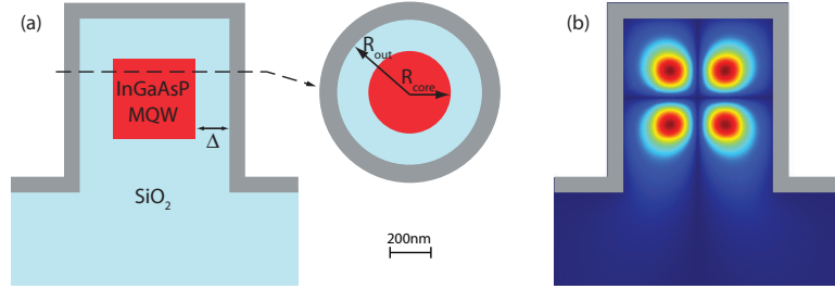
Figure 4.2: (a) Schematic drawing of the wafer bonded metallo-dielectric resonator design; (b) FEM simulation of TE_{012} mode in metallo-dielectric resonator with R_{\text{out}} = 460 \text{ nm} , optimized for 1,550 \text{ nm} wavelength.
