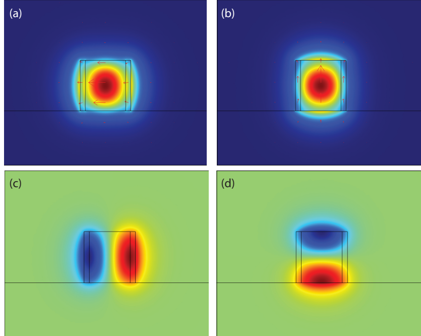
Figure 5.4: COMSOL simulations of fundamental propagating modes in a silicon waveguide. Normal electric field distribution in (a) TE-like mode and (b) TM-like mode. Tangential electric field, E_z component, in (c) TE-like mode and (d) TM-like mode.
