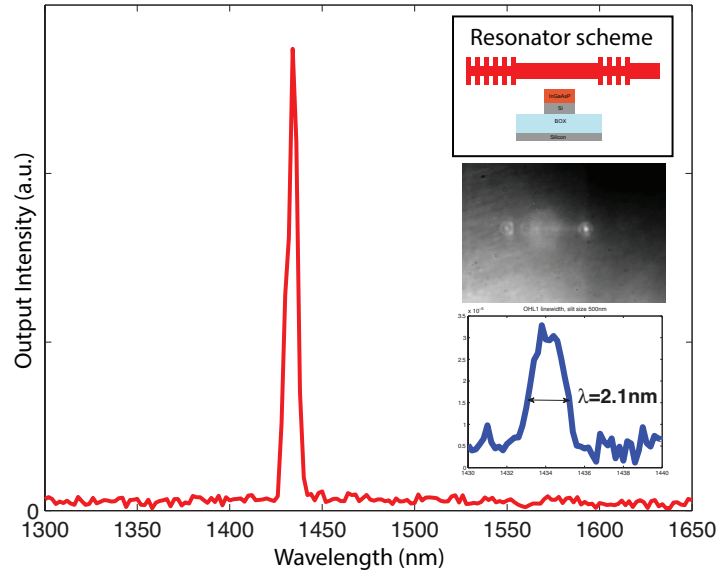
Figure A.1: Optical measurements results of a hybrid III-V/Si DBR laser.
