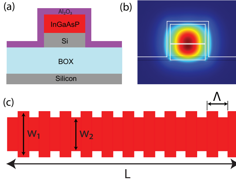
Figure 7.1: III-V/Si hybrid DFB laser design: schematic drawing of a III-V/Si DFB laser resonator with vertical sidewall modulated Bragg gratings – cross-section (a) and top view (c); (b) finite element simulation (COMSOL) of a fundamental TE-like mode for a 500 nm wide and 550 nm tall III-V/Si waveguide with 250 nm silicon layer, 300 nm InGaAsP MQW layer and 50 nm \text{Al}_2\text{O}_3 cladding.
